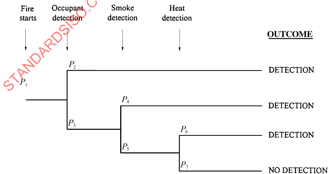
Figure 5 — An event tree
