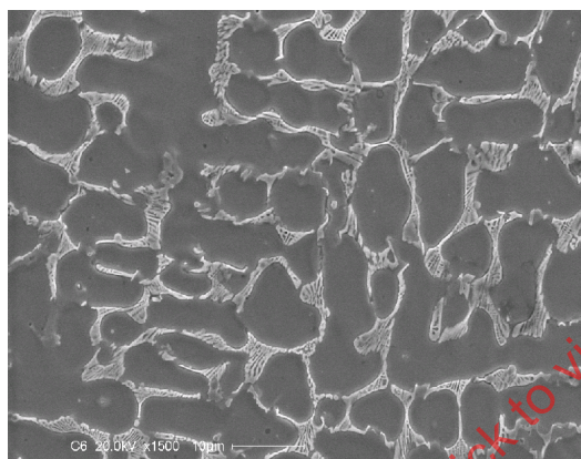
Back-scattered electron image, \times 1\ 500
