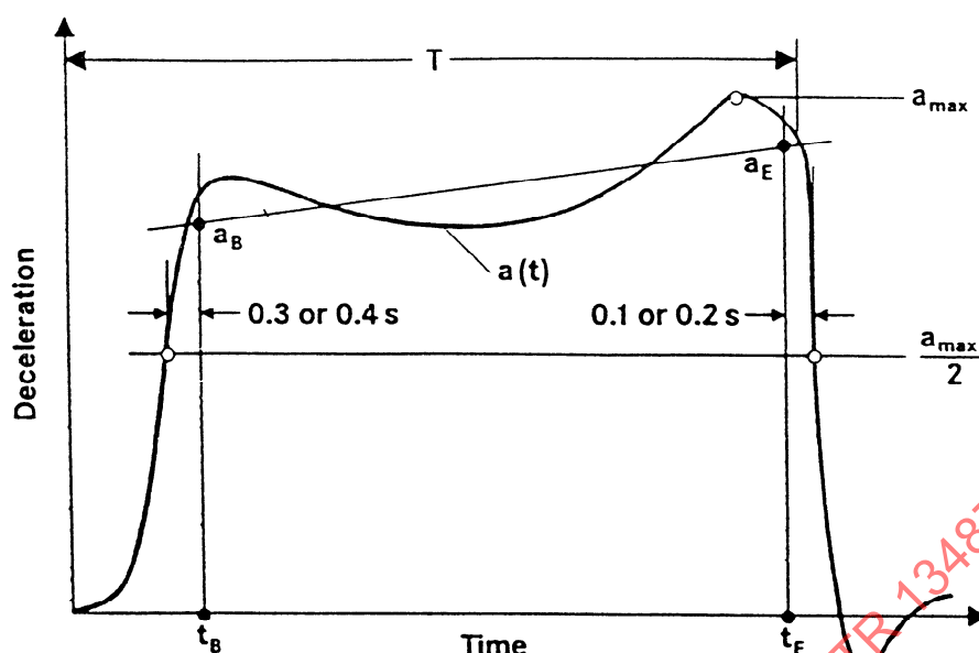
Figure 6 - Determination of the evaluation limits in connection with a time-dependent deceleration path
