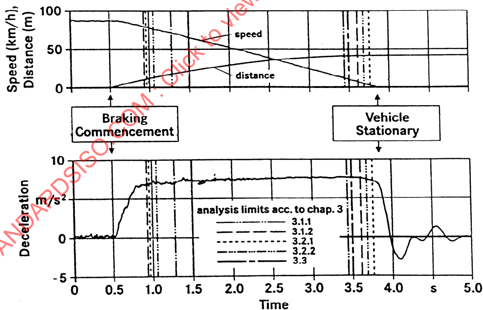
Figure 5 - Analysis limits drawn in time signals of a braking test
