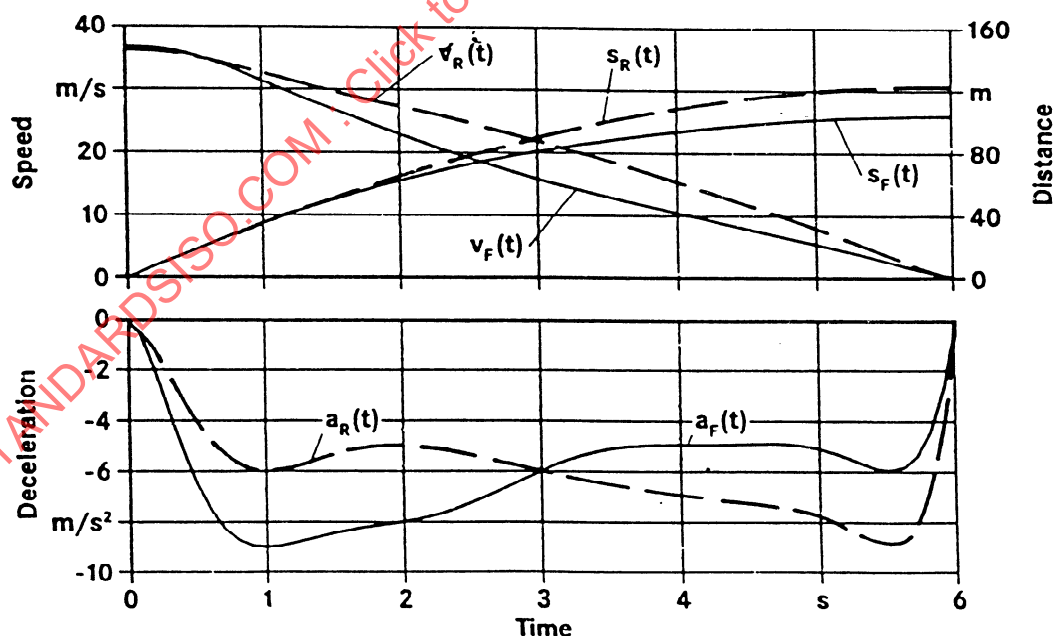
Figure 7 - Analytical functions simulating two different braking processes
