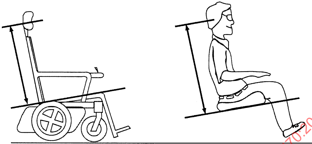
Figure 18 — Headrest height
