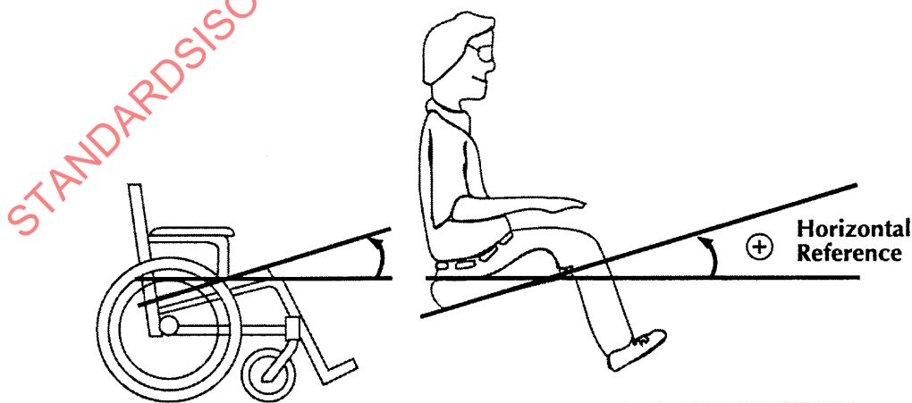
Figure 20 — Seat-plane angle
