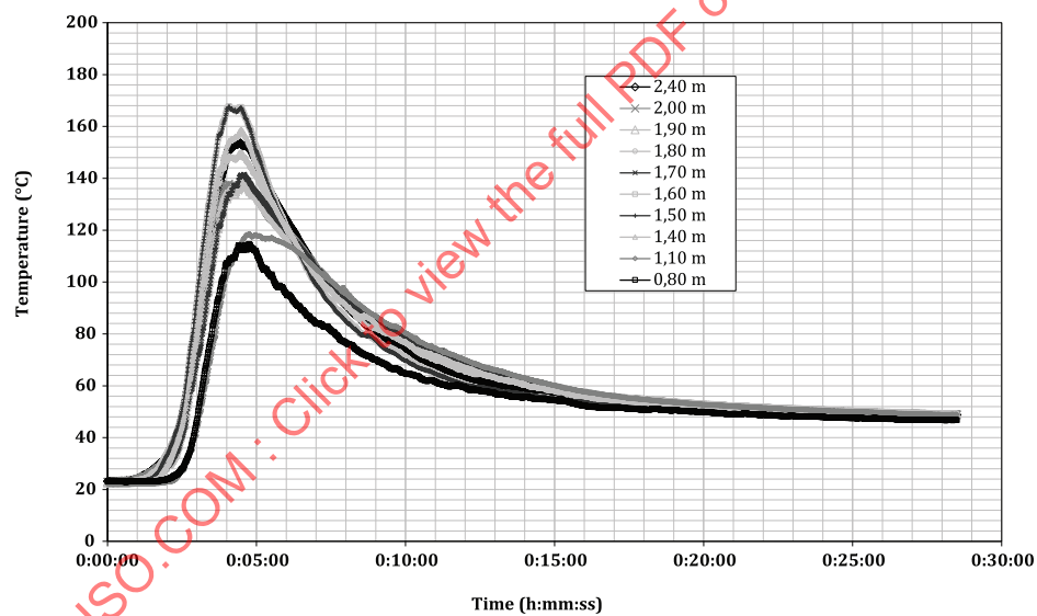
b) Temperature tree, point ATC4 (close to the window)
