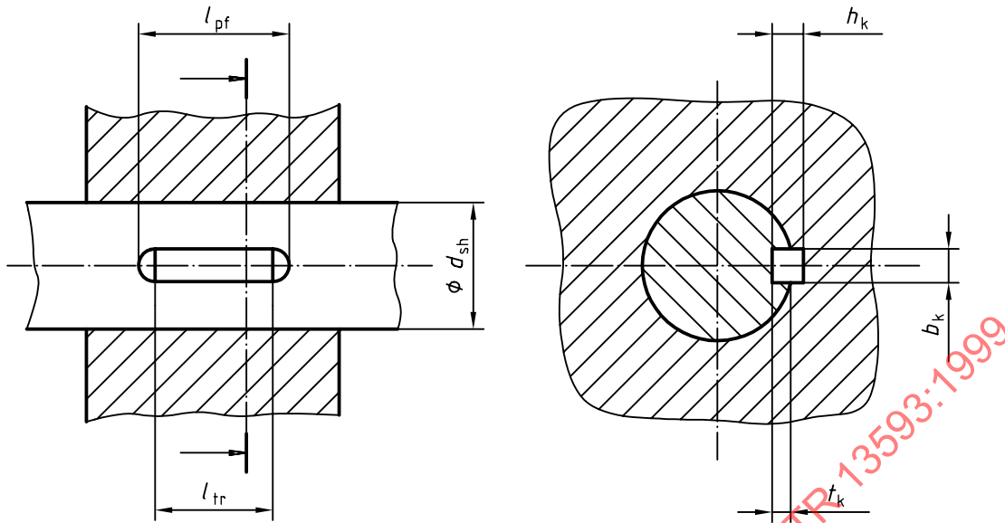
Figure 1 — Fitted key
