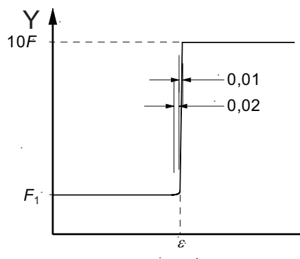
b) Non-linear force/strain relationship
