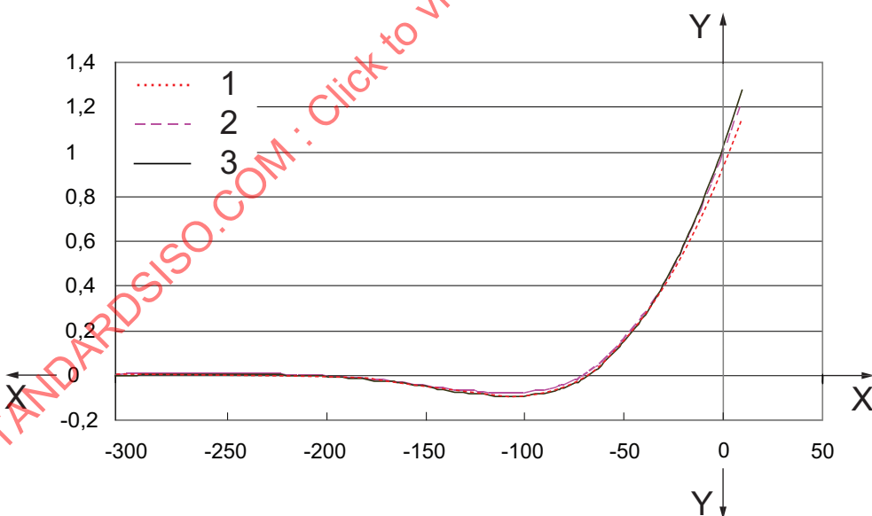
Figure 12 — Envelope of bending moment for coupled model with bending moment from decoupled model superimposed
