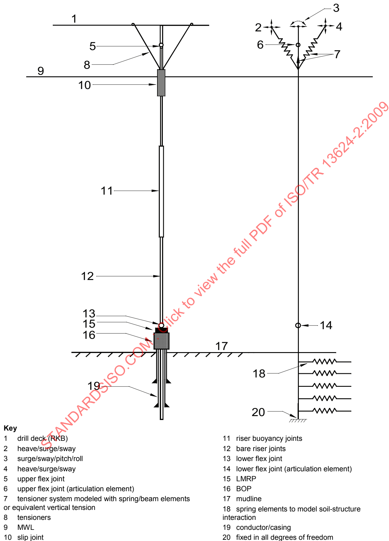
Figure 1 — Drilling riser system configuration and coupled analysis model
