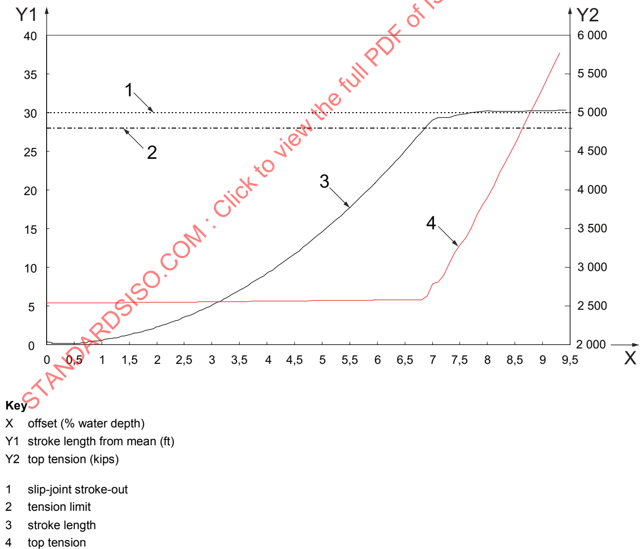
Figure 19 — Stroke length from mean and top tension as a function of offset
