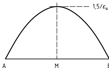
Figure 15 — Load sharing factor for bevel gears with optimal profile modification
