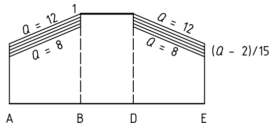
Figure 5 — Load sharing factor for cylindrical spur gears with unmodified profiles and quality grade 7 or finer
