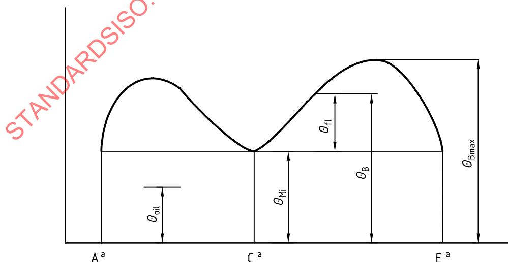
Figure 2 — Contact temperature along the path of contact
