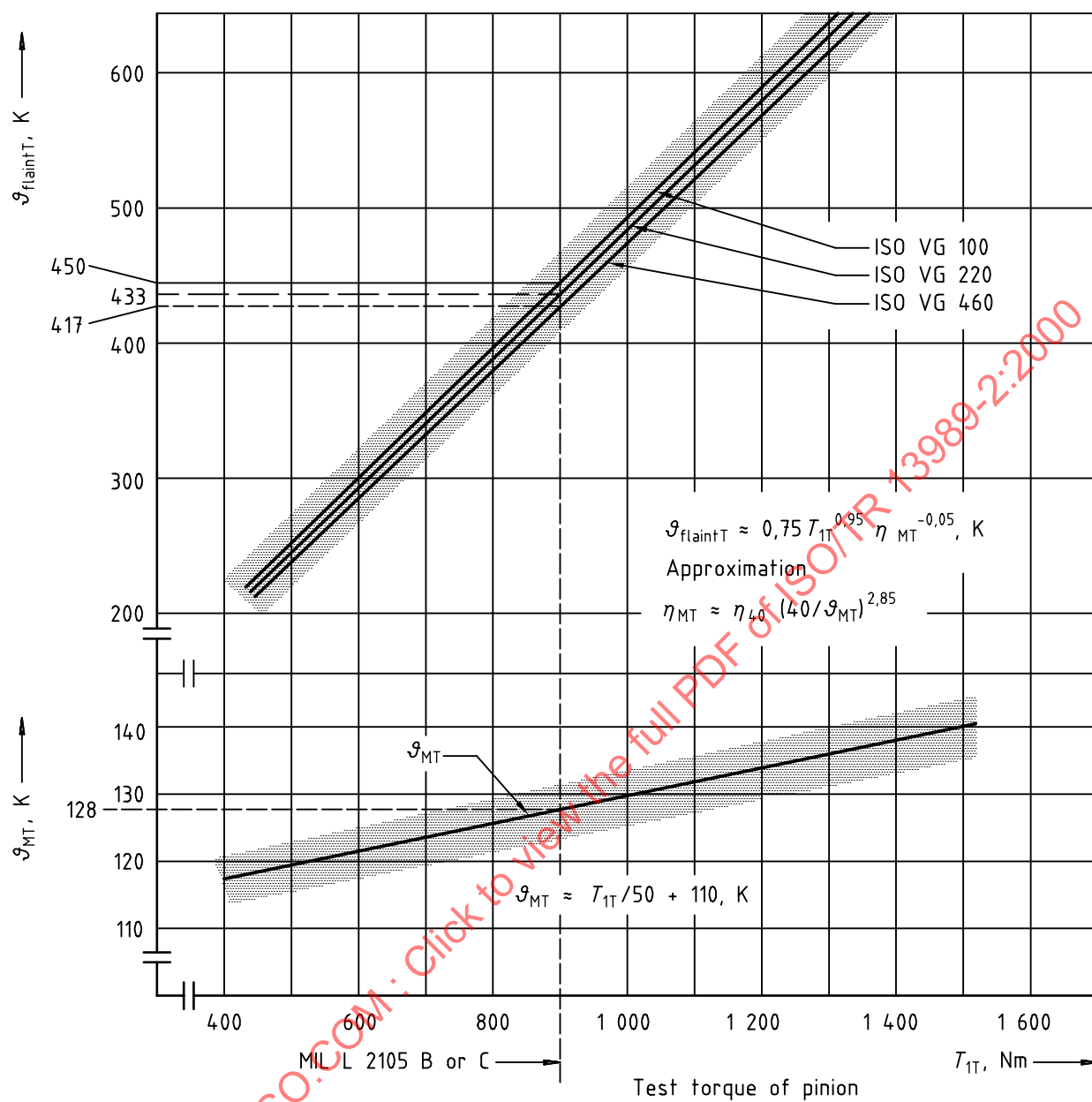
Figure 11 — Scuffing temperature T_{sT} for the FZG L-42 test 141/19,5/110
