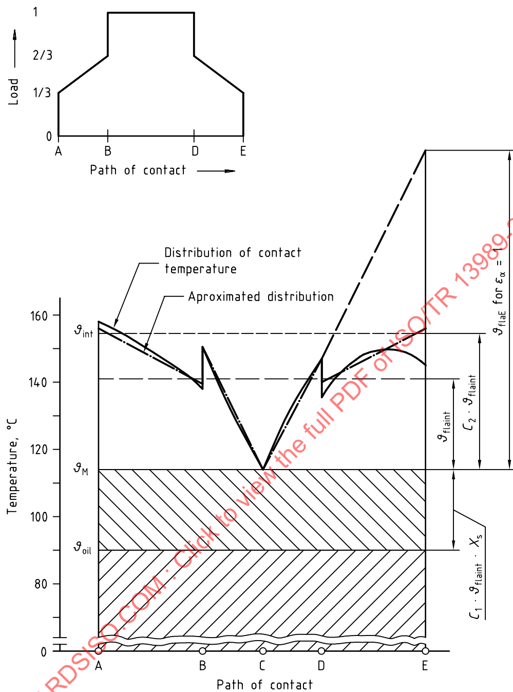
Figure 5 — Load and temperature distribution for 1,0 \leq \varepsilon_{\alpha} < 2,0
