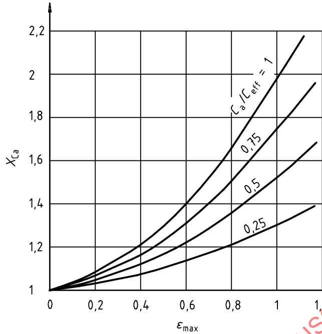
Figure 4 — Tip relief factor X_{Ca} due to experimental data [8, 9]
