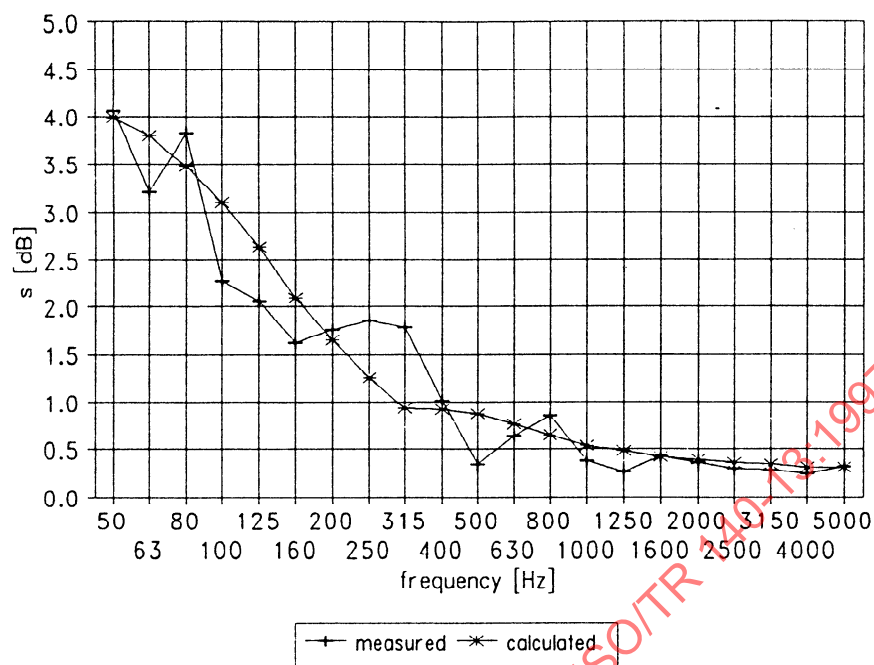
Figure 4.3. Measured and calculated spatial standard deviation of the sound pressure level in room 2.
