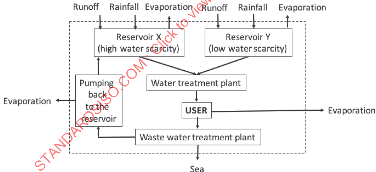
Figure 5 — Option for the supply of water to user
