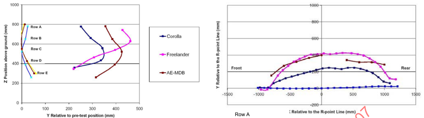
Figure 23 — Static crush of Alfa 147 in several side impact tests [Ellway, 2005]
