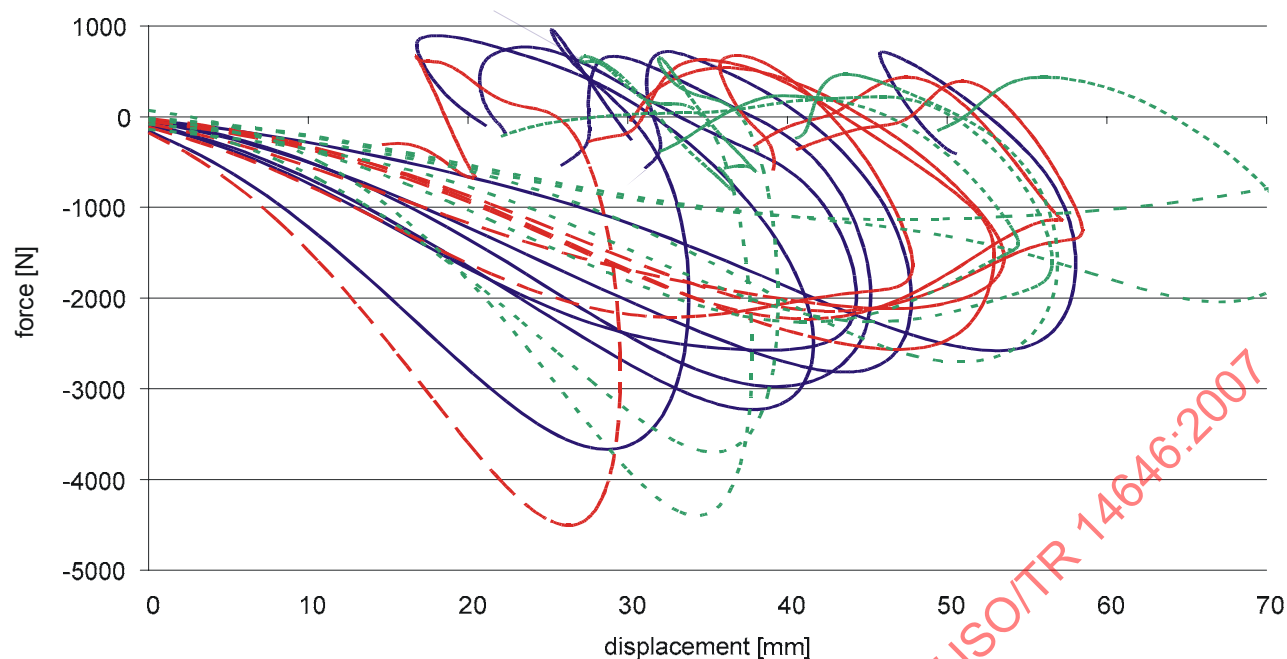
Figure 25 — Door trim force-deflection characteristics of different locations at different doors [Nett, 2003]
