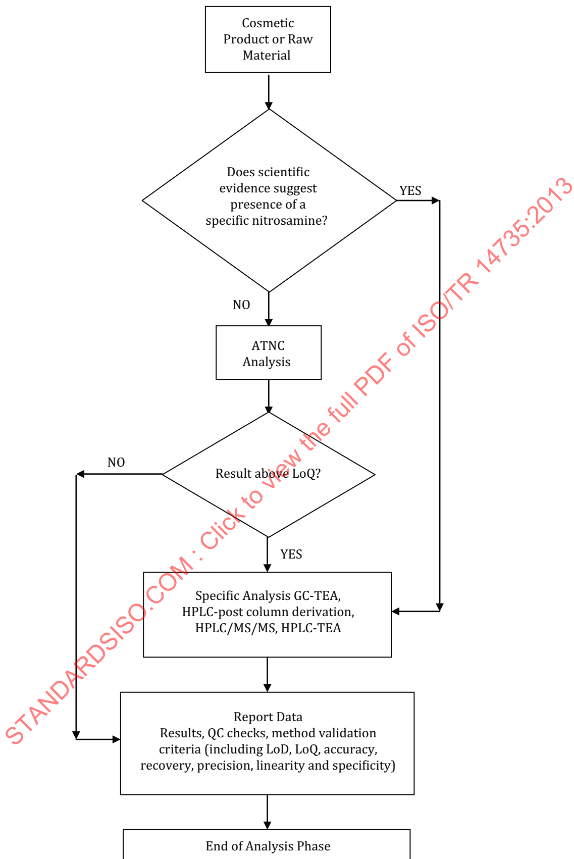
Figure 1 — Analysis of cosmetic products and raw materials (flowchart)
