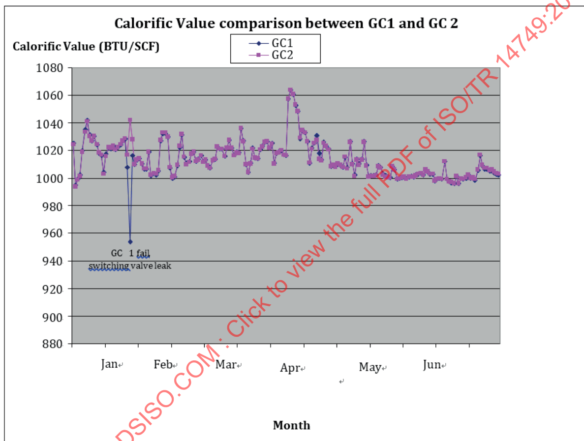
Figure 1 — Comparison between GC1 and GC2 for C7+ application
