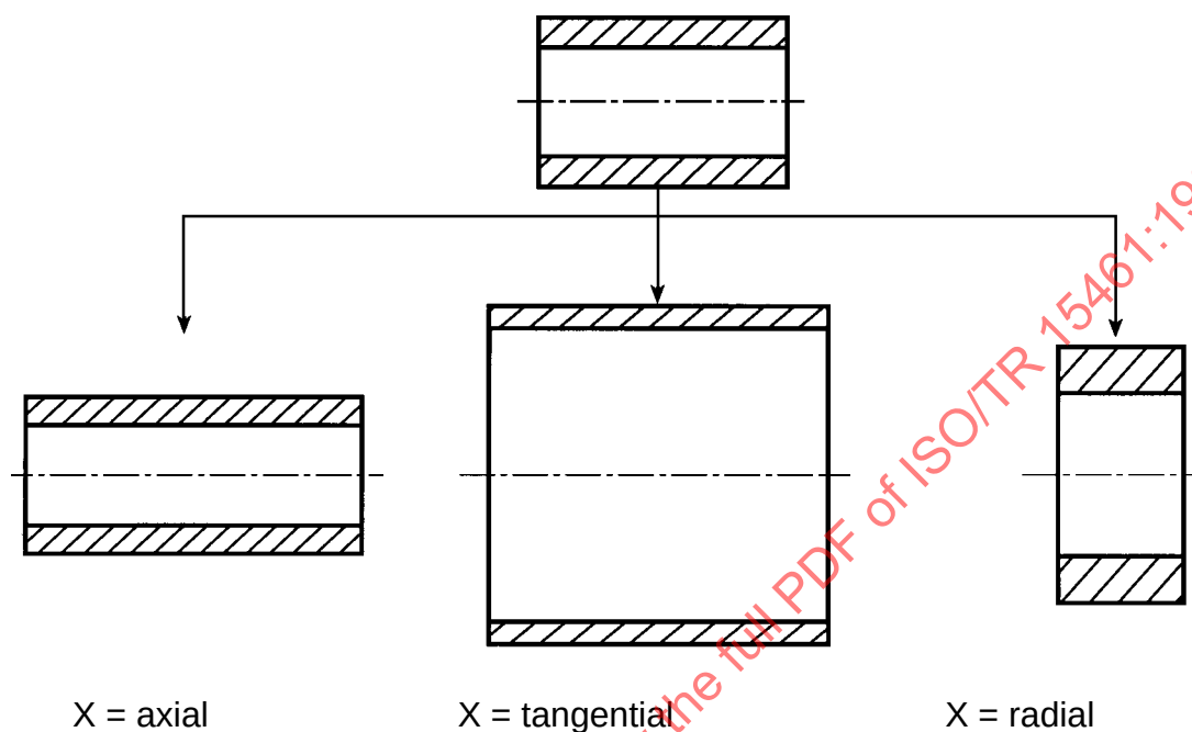
Figure B.1 — Example of the dependance of the X direction on greatest positive strain from the type of forming
