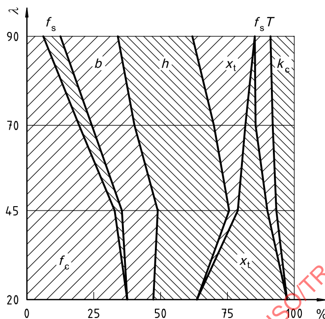
Figure 3 — Separation of total variance in resistance or load-bearing capacity R into component variances as a function of slenderness ratio \lambda for an eccentrically compressed, reinforced concrete column
