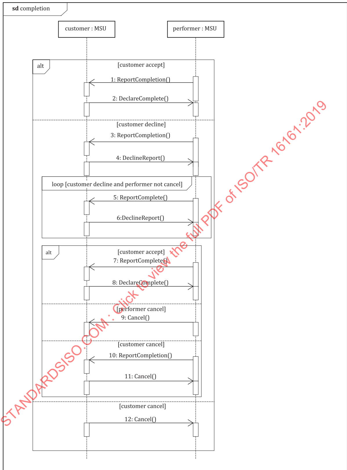
Figure B.7 — Sequence diagram of completion
