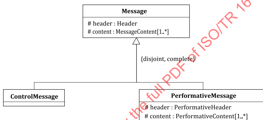
Figure 3 — Structure of Message
