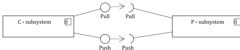
Figure 8 — Interface between C-subsystem and P-subsystem without Notify interface
