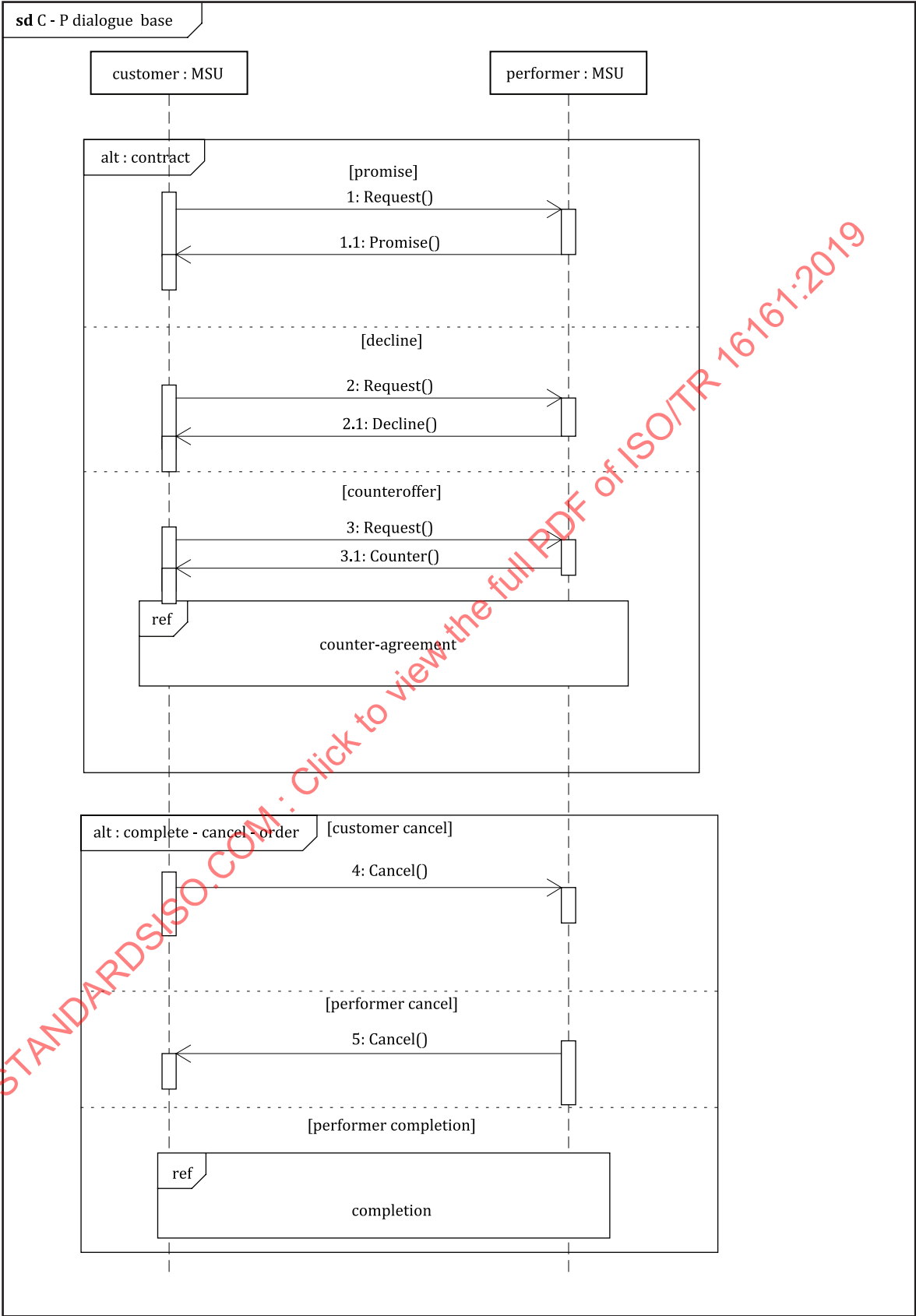
Figure B.5 — Sequence diagram of C-P dialogue base
