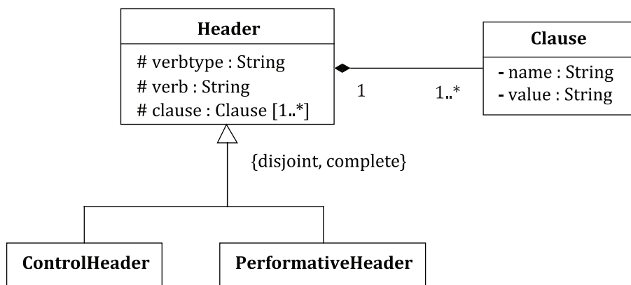
Figure 4 — Structure of Header
