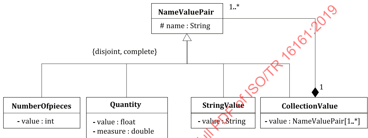
Figure 7 — Structure of NameValuePair
