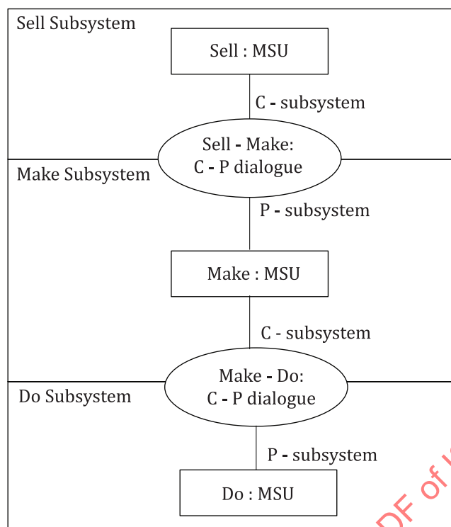
Figure B.4 — Instances of C-P dialogue between Sell Subsystem and Make Subsystem and between Make subsystem and Do Subsystem
