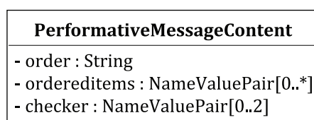
Figure 6 — Structure of PerformativeMessageContent
