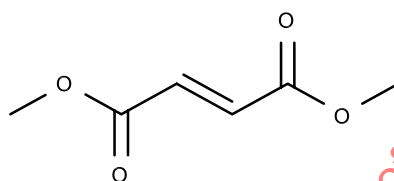
Figure B.4 — Dimethylfumarate molecular structure
