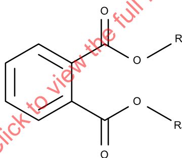
Figure B.12 — Phthalates molecular structure
