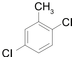
a) Example of chlorotoluene molecular structure
