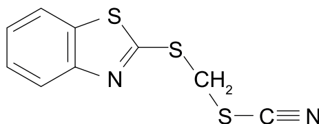
Figure 6 — TCMTB molecular structure
