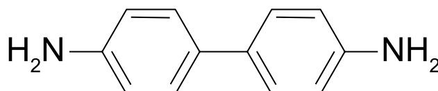
a) Example of aromatic amines molecular structure; benzidine
