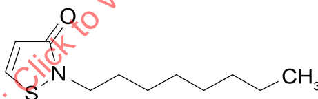
Figure 7 — OIT molecular structure
