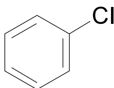
b) Example of chlorobenzene molecular structure
