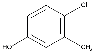
Figure 8 — CMK molecular structure
