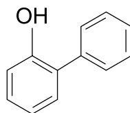
Figure 5 — Orthophenylphenol molecular structure
