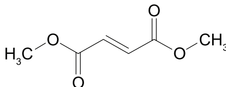
Figure 14 — Dimethylfumarate molecular structure
