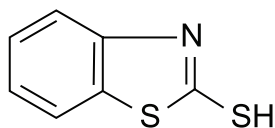
Figure 16 — Mercaptobenzothiazole molecular structure
