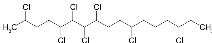
Figure 10 — Example of a Chlorinated paraffins molecular structure
