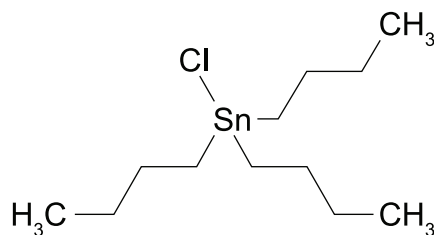
Figure 21 — Example of organotin molecular structure
