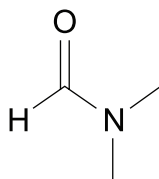
Figure 13 — Dimethylformamide molecular structure
