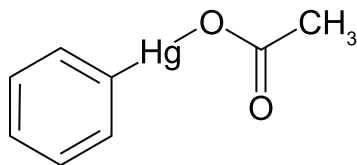
Figure 26 — Example of phenyl mercury component acetate phenylmercury
