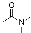
Figure 19 — N,N-dimethylacetamide molecular structure
