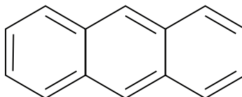
Figure 22 — Example of PAH structure, Anthracene
