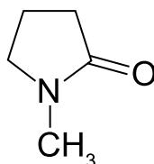
Figure 18 — N-methyl-2-pyrrolidone molecular structure
