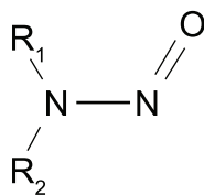
Figure 20 — Nitrosamines molecular structure
