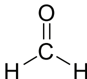
Figure 15 — Formaldehyde molecular structure
