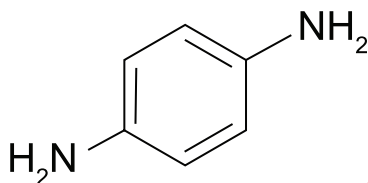
Figure 23 — Paraphenylene diamine molecular structure
