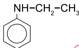
Figure 17 — N-ethylphenylamine molecular structure
