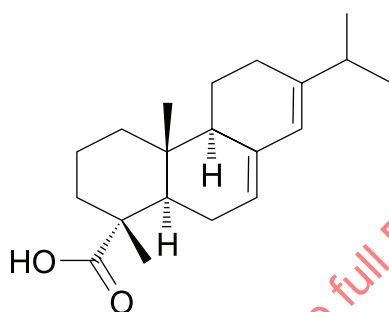
Figure 12 — Example of a colophony component molecular structure, abietic acid
