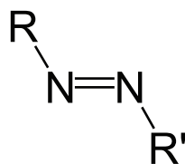
b) Molecular structure of the azo function
