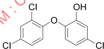
Figure 9 — triclosan structure
