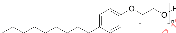
Figure 2 — Example of Alkylphenol ethoxylates molecular structure, nonylphenol ethoxylate
