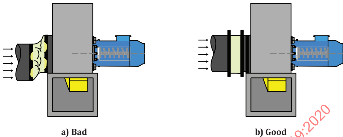
Figure 31 — Inlet blockage example
