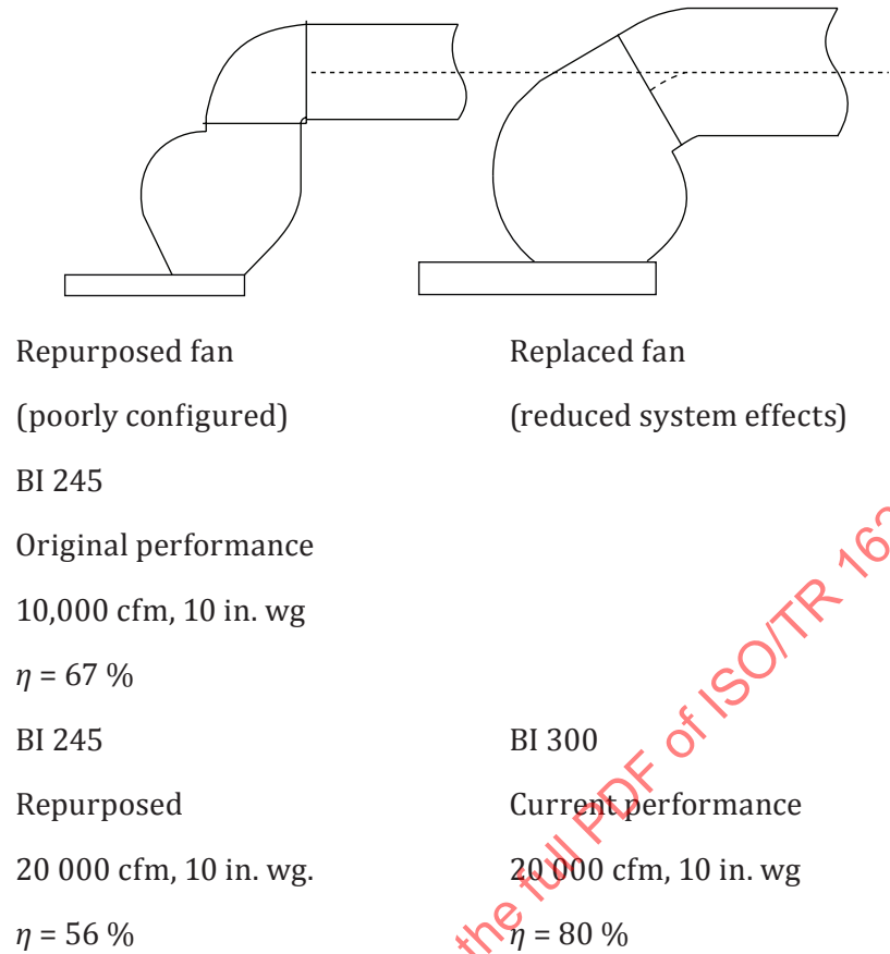
Figure 40 — Fan replacement of a poorly configured fan
