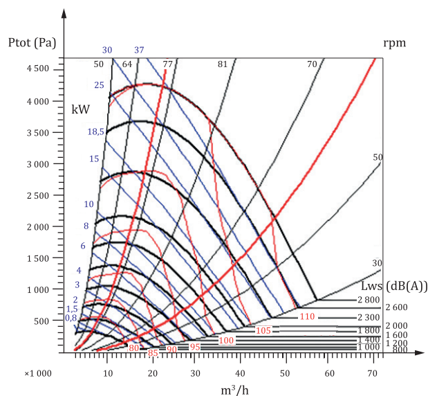
Figure A.4 — Family of constant-speed curves on linear scales
