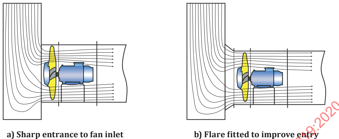
Figure 29 — Examples of fan inlet entrances to a fan inlet
