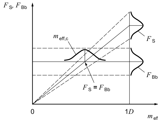
Figure 3 — Relation among the fracture loads ( F_S and F_{Bb} ) and the effective nut height ( m_{eff} )
