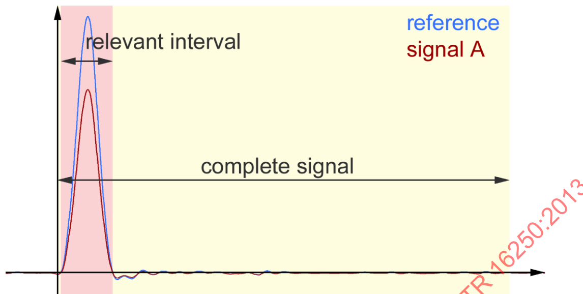
Figure 13 — Different intervals of evaluation [10]
