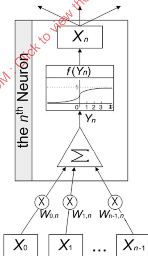
Figure B.2 — Simple neural network
