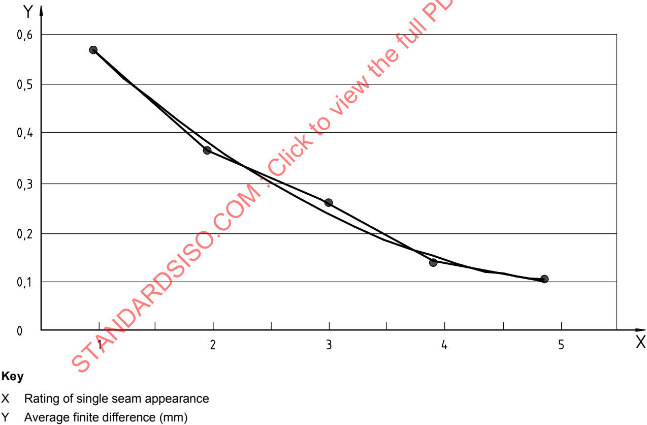
Figure A.3 — Rating of standard 3-D replica vs seam pucker information of finite difference algorithm
