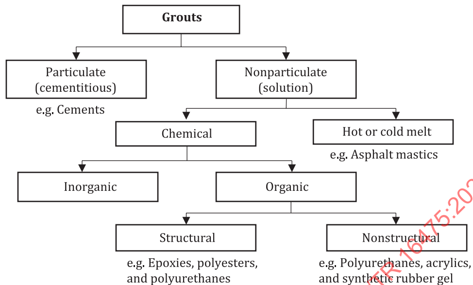
Figure 3 — Classification of grout material types
