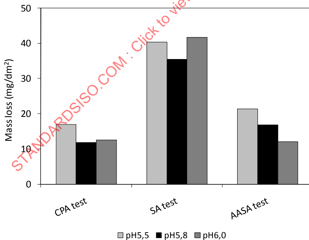
Figure 12 — Comparison of the mass loss for cold sealing at 30 °C and for 0,75 min/μm with different pH values
