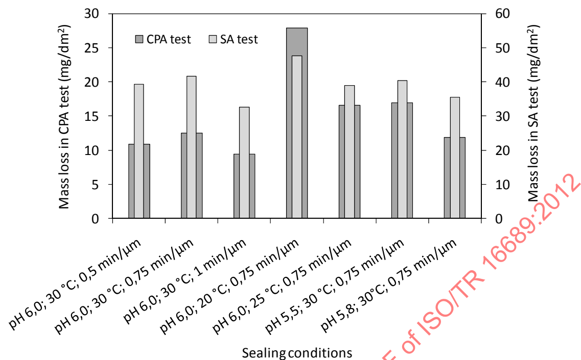
Figure 15 — Relative comparison of the mass loss for the CPA test and the sulfuric acid test
