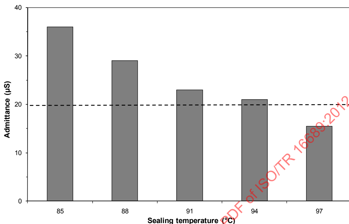
Figure 10 — Admittance of 20 μm thick coatings sealed with hot sealing at different temperatures
