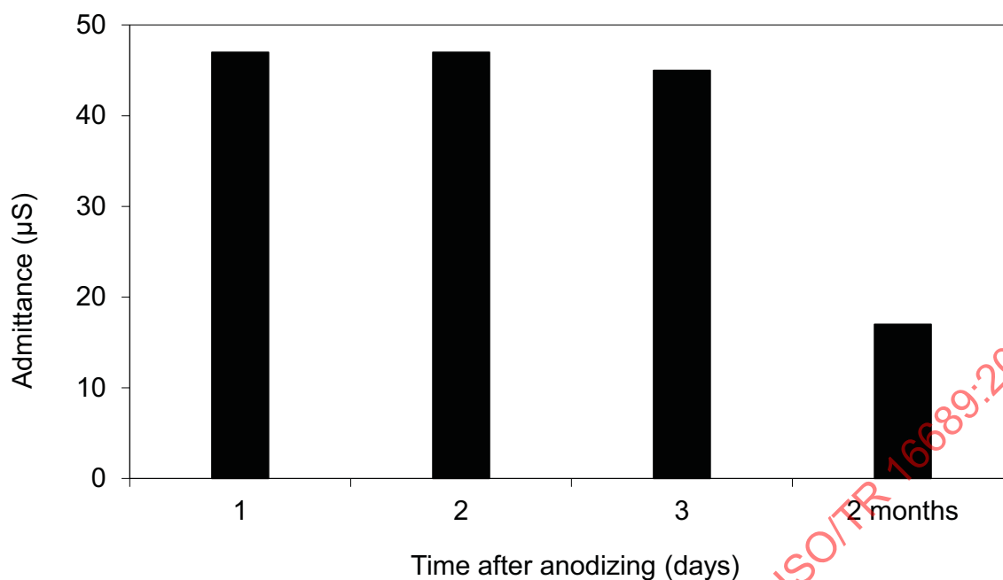
Figure 25 — Admittance of 10 μm thick coatings measured at various times after sealing with nickel-free midtemp sealing for 3 min/μm [18]
