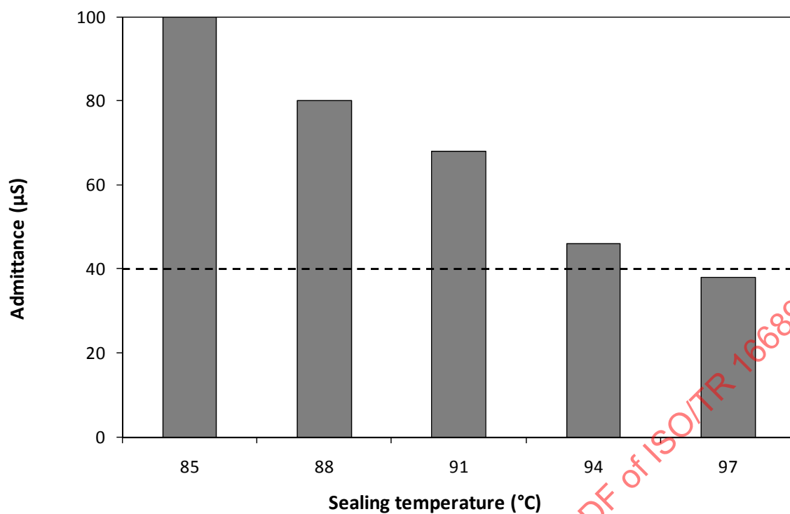
Figure 8 — Admittance of 10 μm thick coatings sealed with hot sealing at different temperatures
