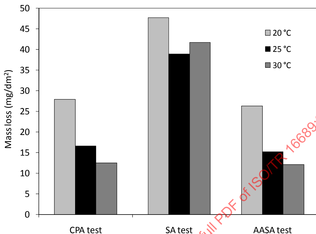
Figure 13 — Comparison of the mass loss for cold sealing at pH 6,0 and for 0,75 min/ \mu m with different temperatures
