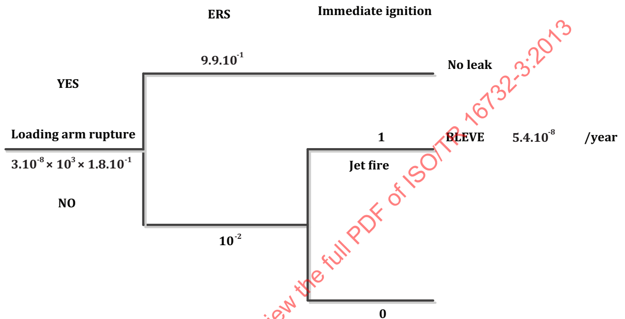
Figure 9 — Event tree for a full-bore rupture jet fire (Option 4)
