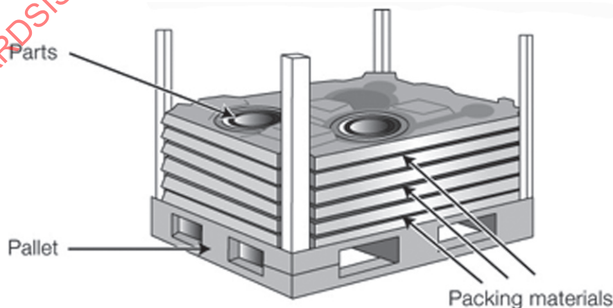
Figure 13 — Packing material
