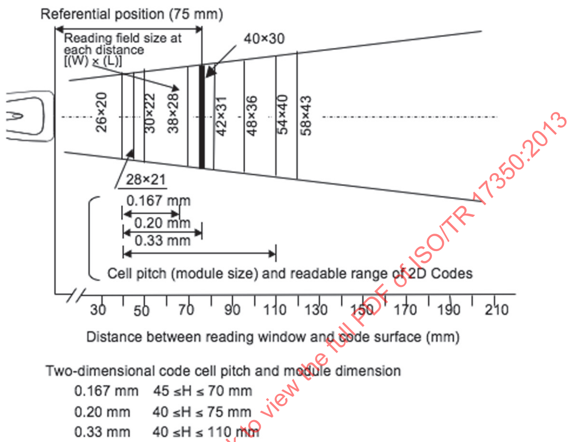
Figure C.2 — Reading specifications of the hand-held scanner used
