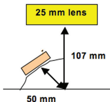
Figure 25 — Evaluation Method 1
