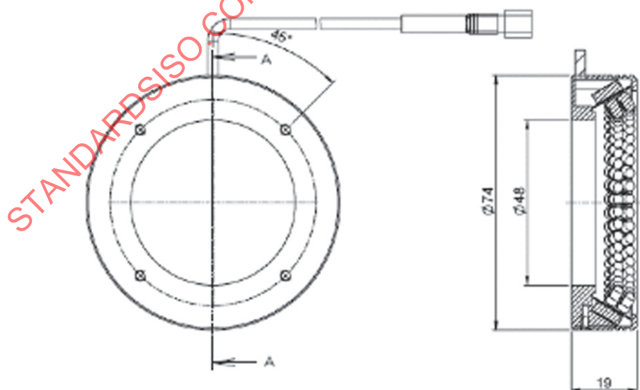
Figure F.1 — Outer dimensions of red-coloured low angle light
