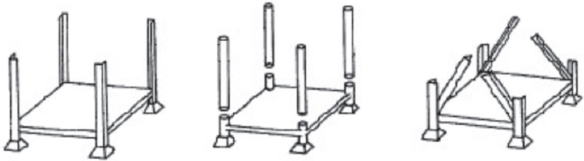
Figure 4 — Post pallets
