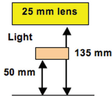
Figure 26 — Evaluation Method 2
