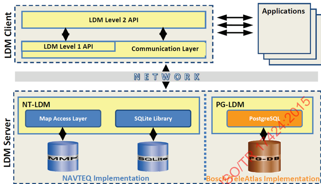
Figure 9 — LDM architecture
