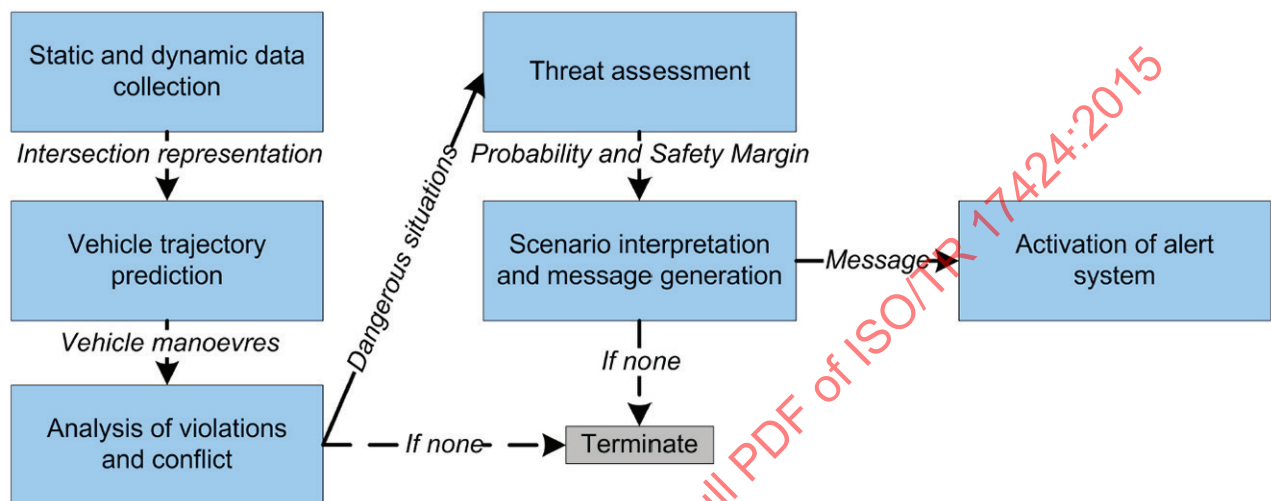
Figure 5 — Functional description of IRIS
