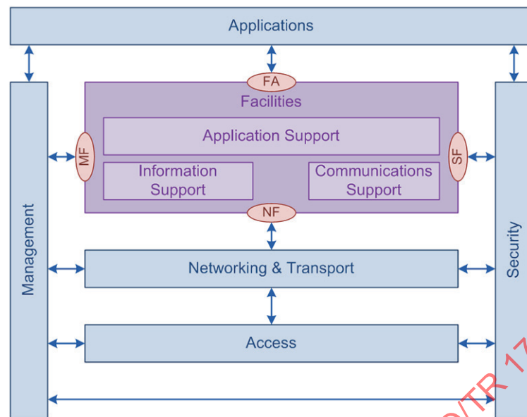
Figure 11 — ITS station reference architecture
