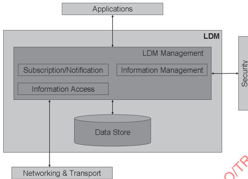
Figure 13 — LDM architecture
