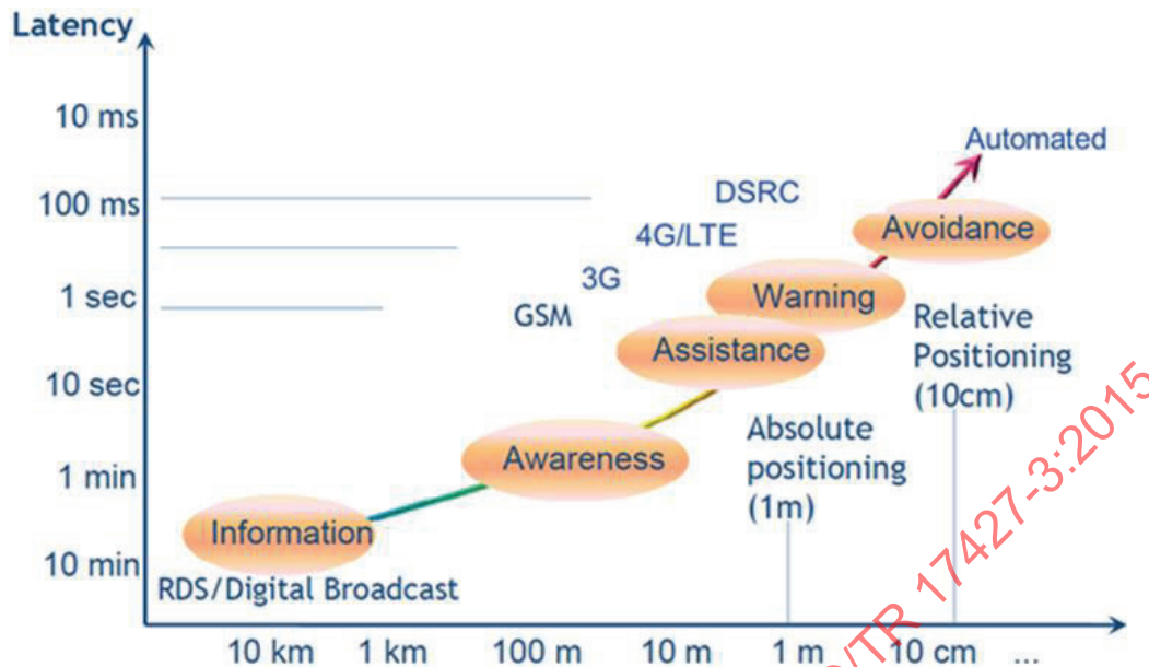
Figure 6 — Types of C-ITS by latency and spatial accuracy [Source: Modified from ERTICO 2011]
