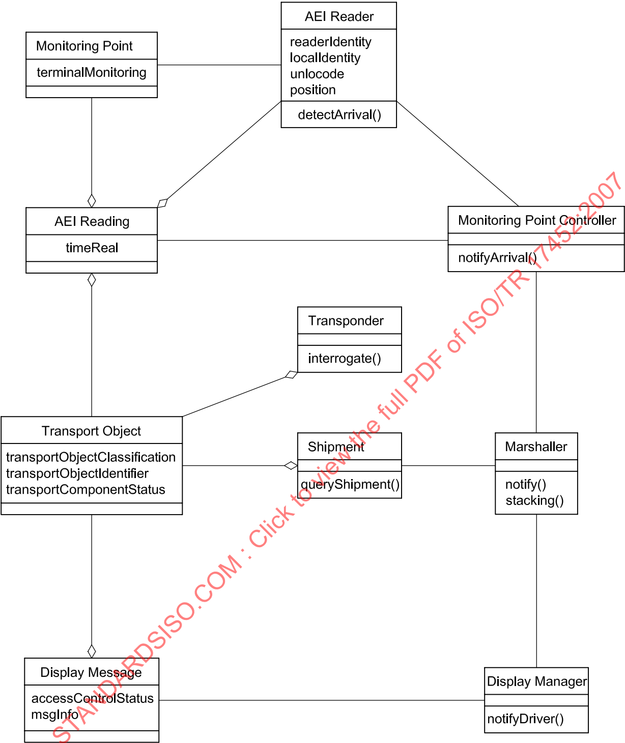
Figure 6 — Information classes and the main classifiers: class attributes
