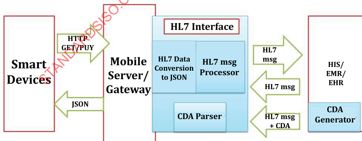
Figure 3 — Mobile electronic medical record system
