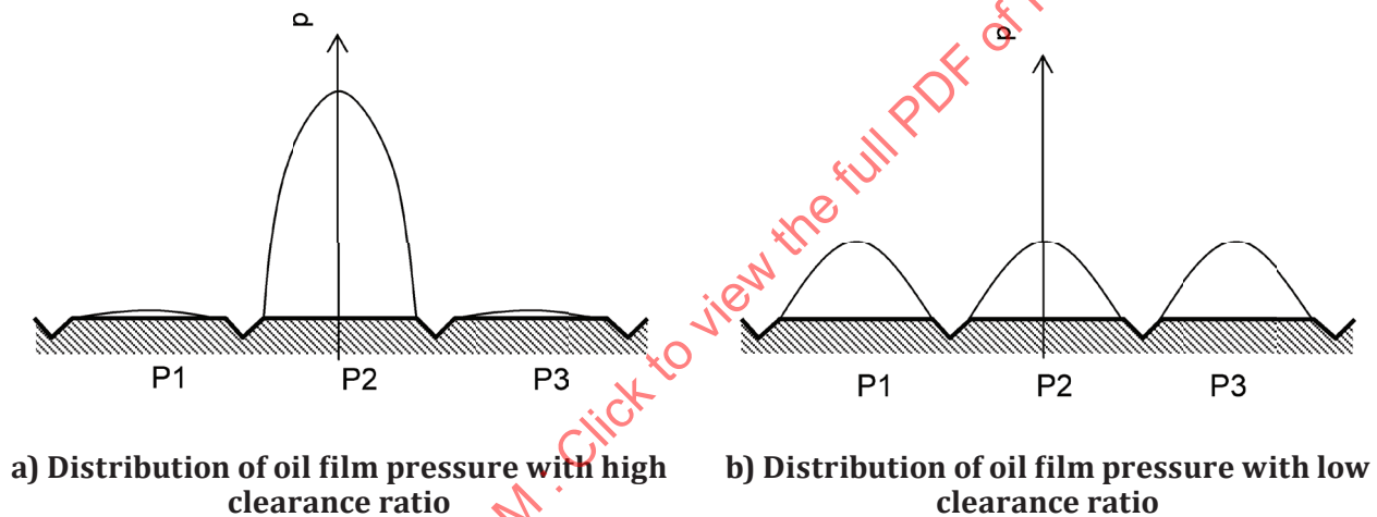
Figure 4 — Distributions of oil film pressure
