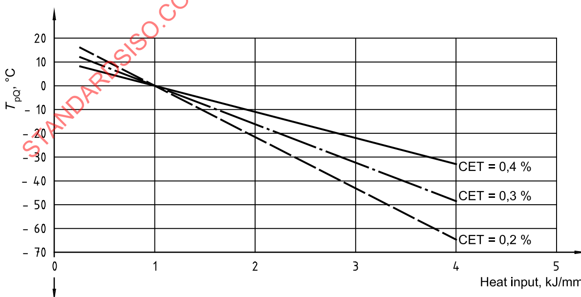
Figure A.6 — Preheat temperature as a function of heat input
