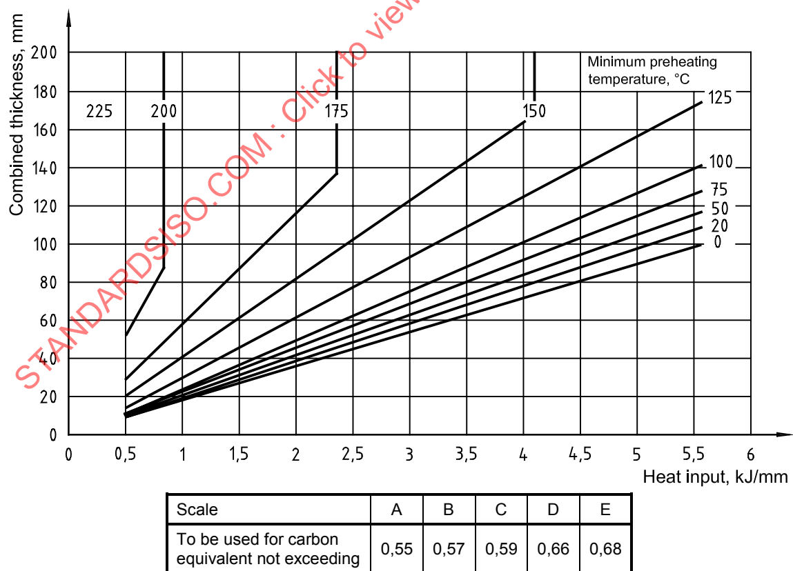
Figure A.2 — Conditions for welding steels with defined carbon equivalents
