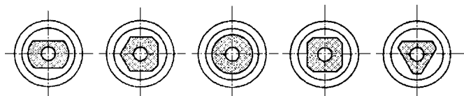
Figure 44 — Coupling sockets
