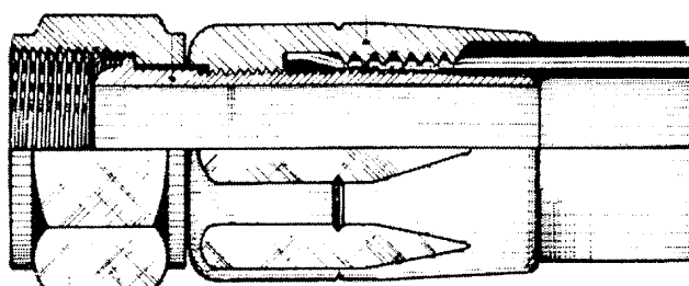
Figure 41 — Threaded sleeve coupling
