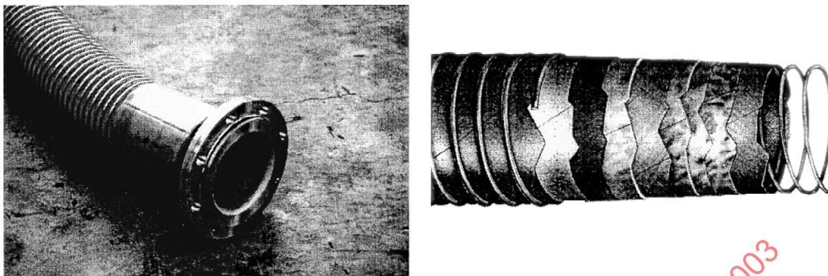
Figure 23 — “Multilayer” or “composite” hose for liquids
