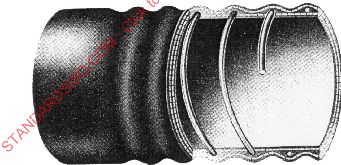
Figure 20 — Wrapped, with embedded spiral and corrugated cover
