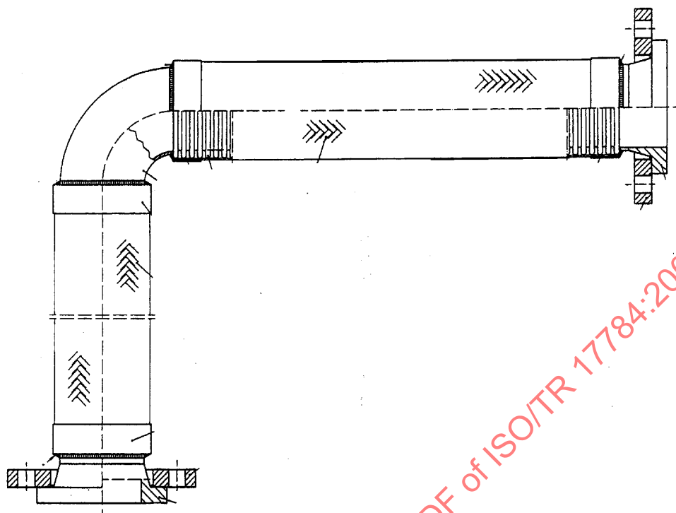
Figure 19 — “Dog-leg” installation
