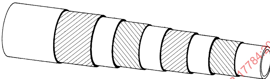
Figure 28 — Hydraulic hose with four spirally wrapped layers
