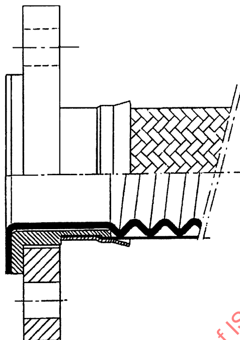
Figure 25 — Protected coupling and sealing surface
