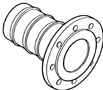
Figure 33 — Hose nipple with beads for assembly by vulcanizing or with clamps
