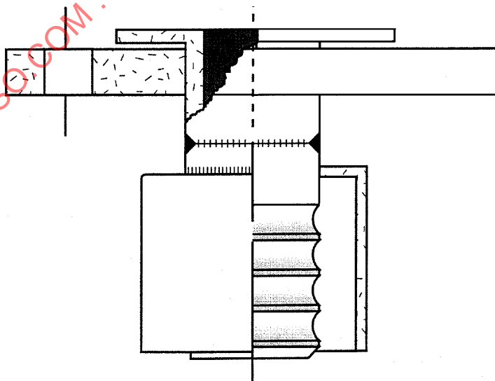
Figure 36 — Flanged connection with externally swaged sleeve
