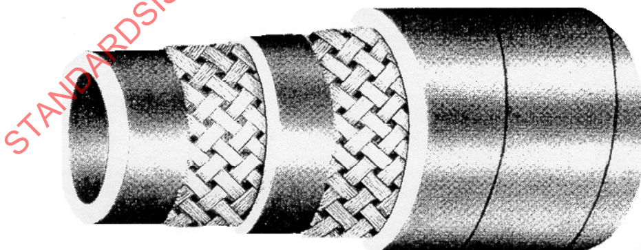
Figure 21 — Cover with cloth imprint
