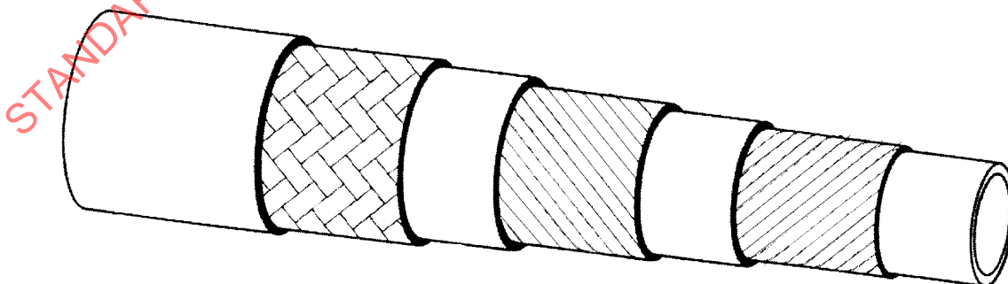
Figure 27 — Hydraulic hose with two spirally wrapped reinforcing layers and one braided reinforcing layer
