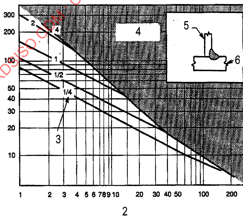
Figure 15a) – Single-pass SAW fillet welds with web and flange of same thickness
