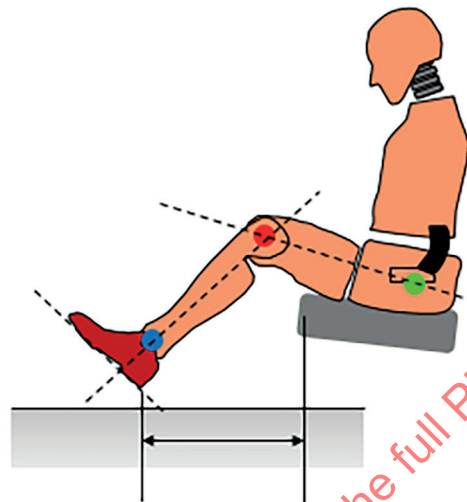
Figure 4 — Lower leg positioning Step 1
