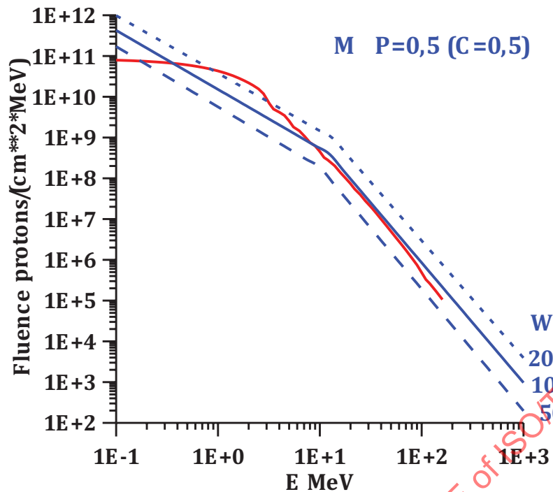
Figure A.6a — Differential energy spectra of annual missions in case of spectra M, P = 0,5 , (or confidence level 0,5 for model ESP) and present model for solar activity, W = 50, 100 , and 200 (model parameters \langle n \rangle = 8, 16 , and 32 )
