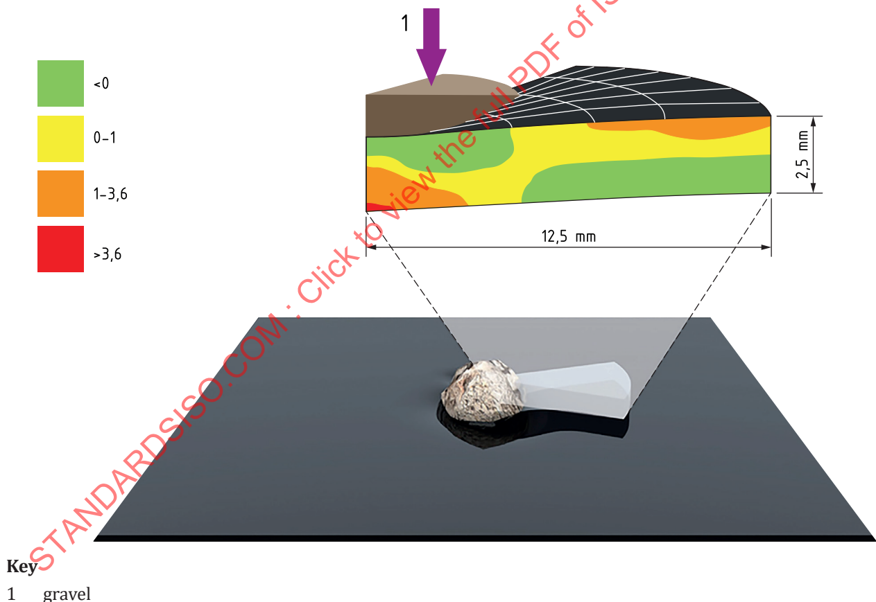
Figure 6 — Elongation in the tangential plane \epsilon_B (%) when \epsilon_L = 0,25 % (picture courtesy of Naue)
