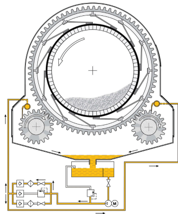
Figure 12 — Circulation lubrication 7)
