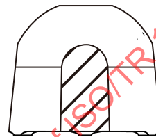
b) Specimen intaglio surface planes in the Z-direction
