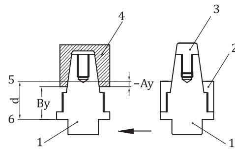
b) Vertical discrepancy (-Ay) measurement of crown without removable parts
