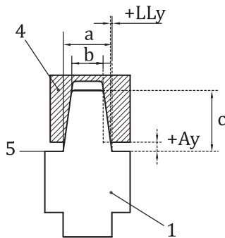
c) Lateral discrepancy (+LLy) of crown with removable parts
