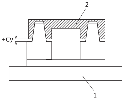
a) Discrepancy measurement with removable parts
