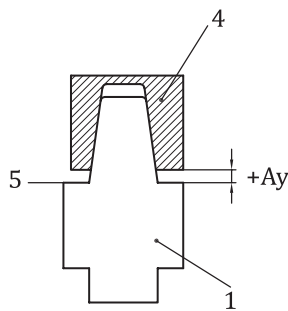
a) Vertical discrepancy (+Ay) measurement of crown with removable parts
