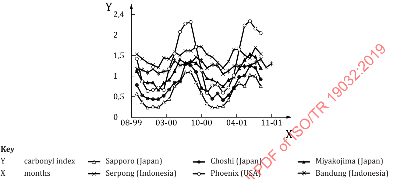
Figure 7 — Behaviour of monthly carbonyl index at each place
