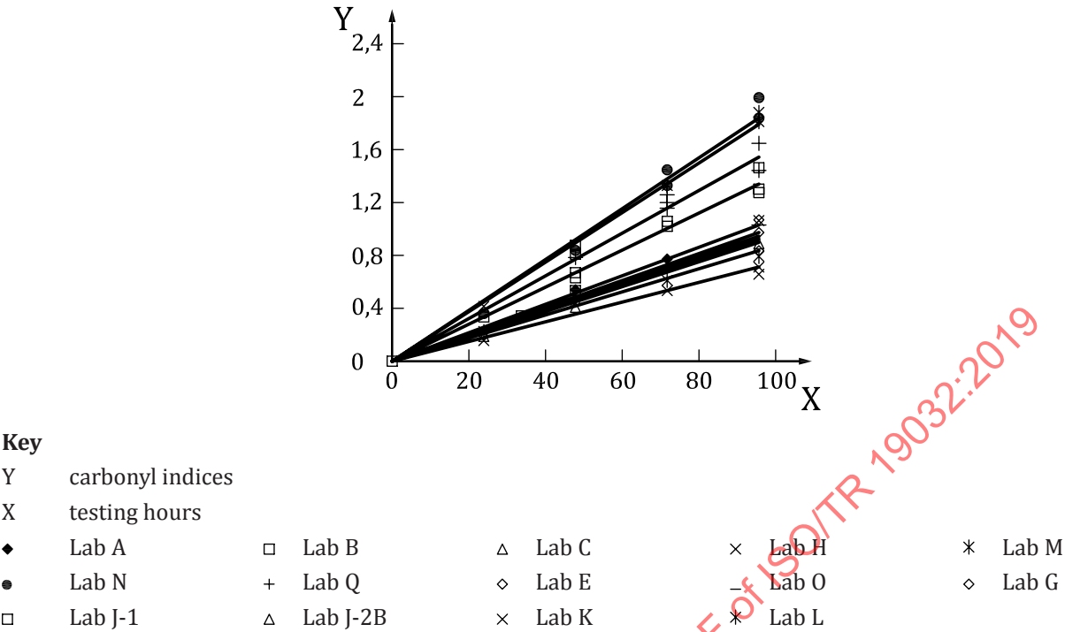
Figure 3 — Summary of xenon-arc exposure
