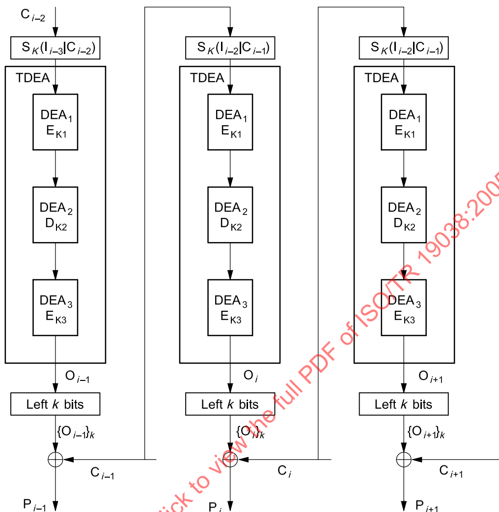
Figure 6 — TDEA cipher feedback-decryption
