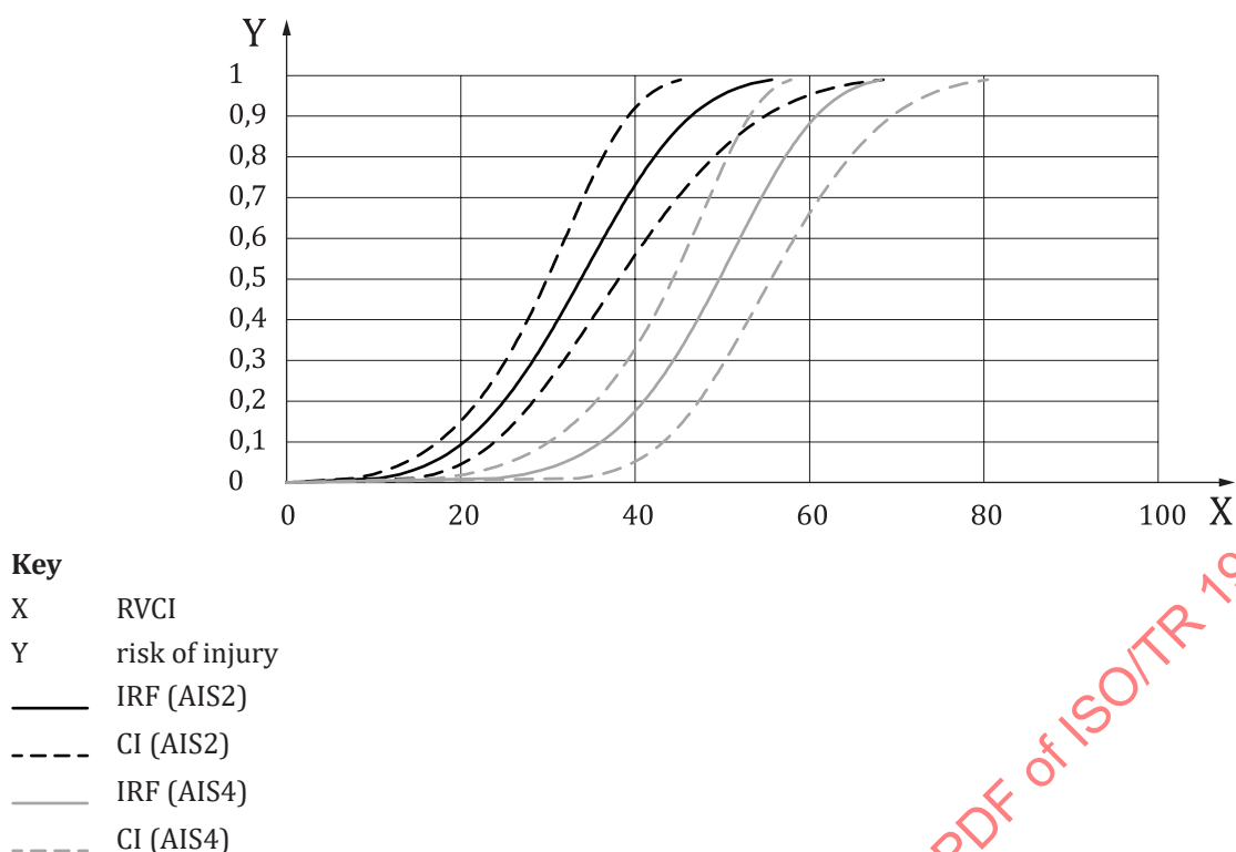
Figure 7 — Injury risk curves for AIS 2 and AIS 4 as a function of RVC I
