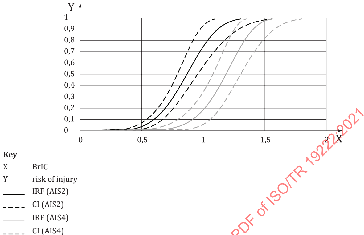
Figure 6 — Injury risk curves for AIS 2 and AIS 4 as a function of BrIC
