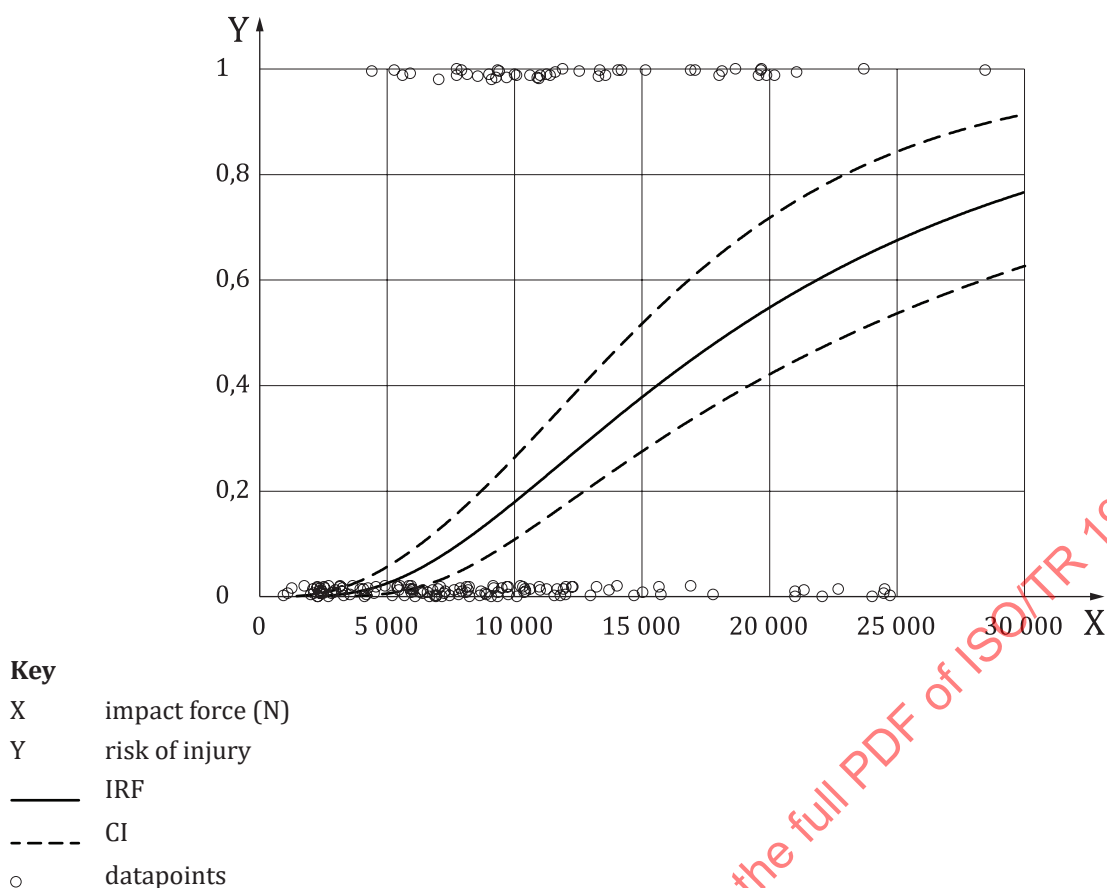
Figure F.4 — Final injury risk curve with 95 % CI at 60 years old, for a padded impact
