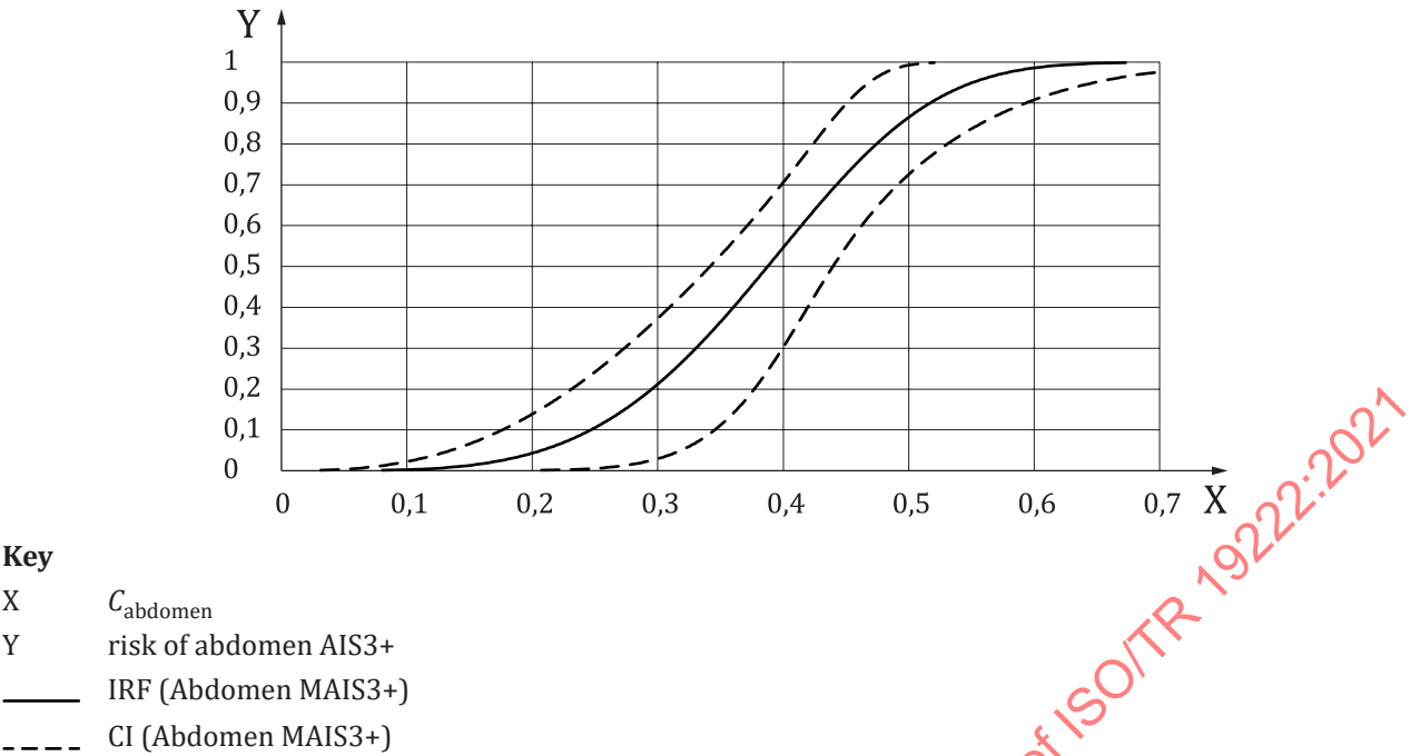
Figure 17 — Injury risk curves for MAIS3+ as a function of C_{\text{abdomen}}
