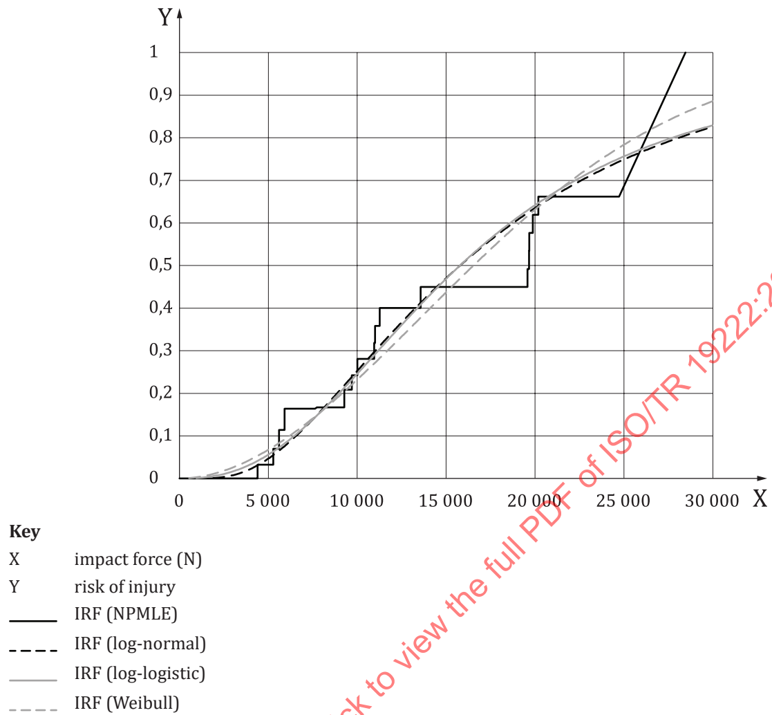
Figure F.3 — Check of distribution assumption of the model
