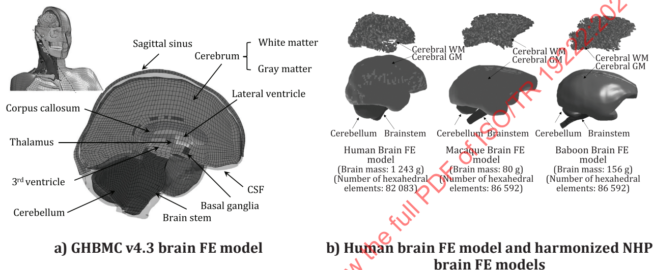
Figure B.1 — Brain FE models used in the construction of IRCs
