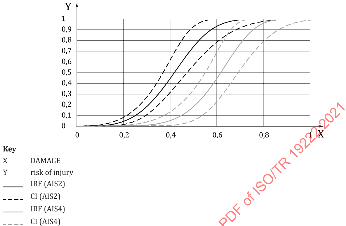
Figure 3 — Injury risk curves for AIS 2 and AIS 4 as a function of DAMAGE
