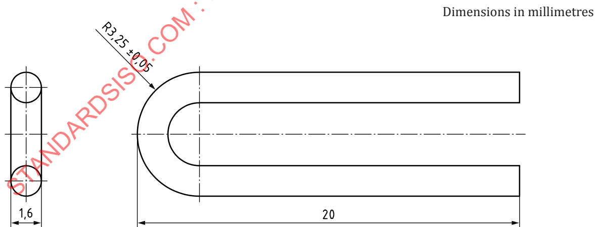
Figure 43 — Test tool (curved stylus)
