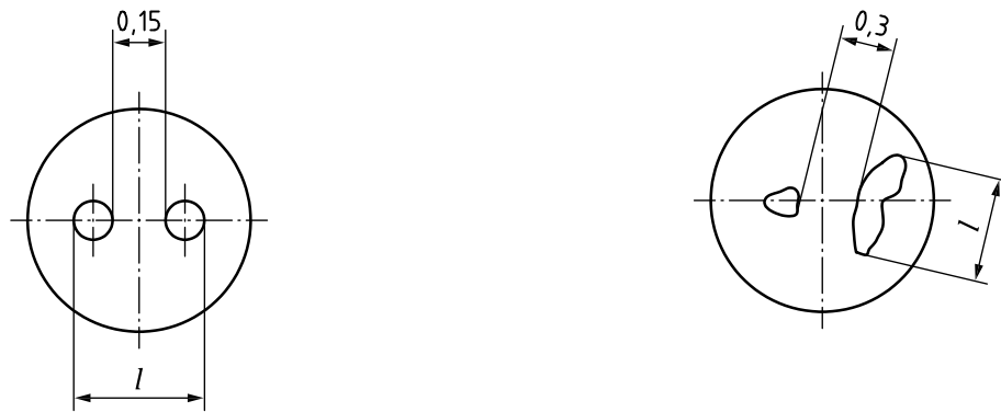
a) Distance between the single defects \leq 0,2 mm
