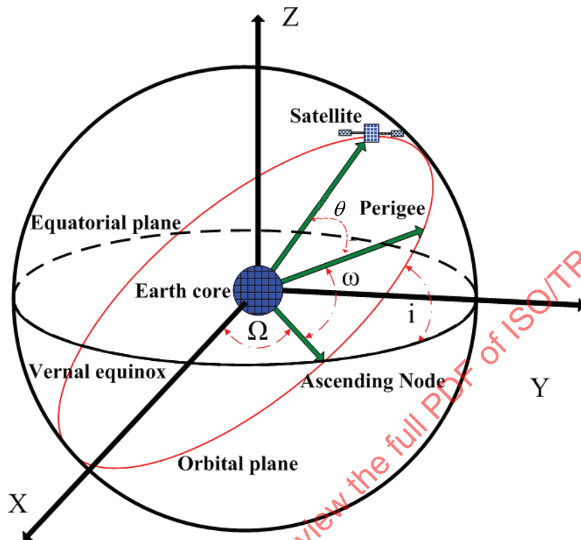
Figure 1 — Orbit elements
