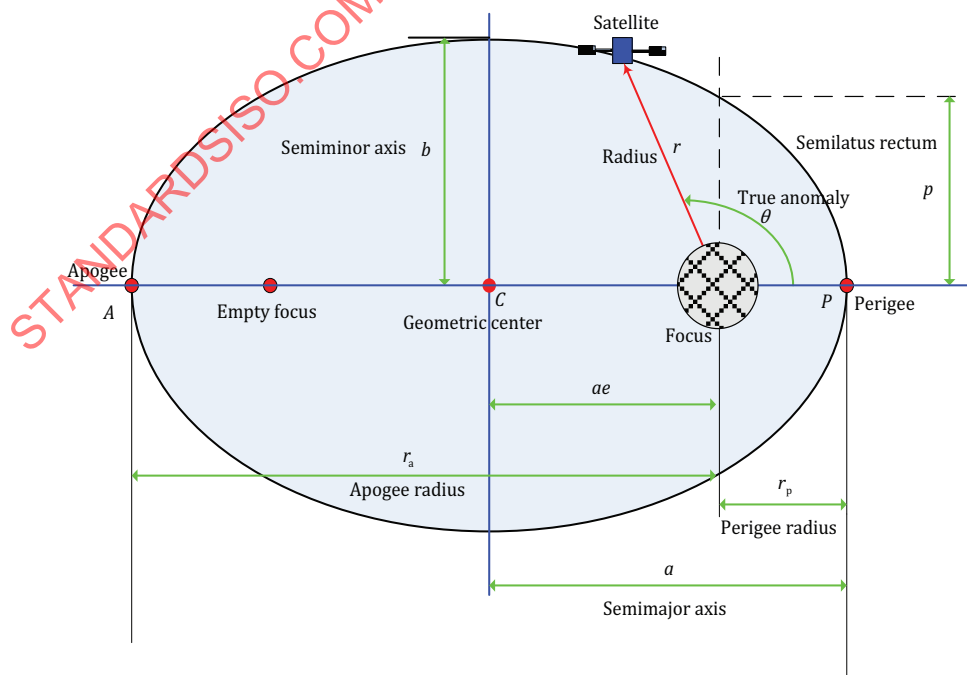
Figure 2 — Ellipse geometry
