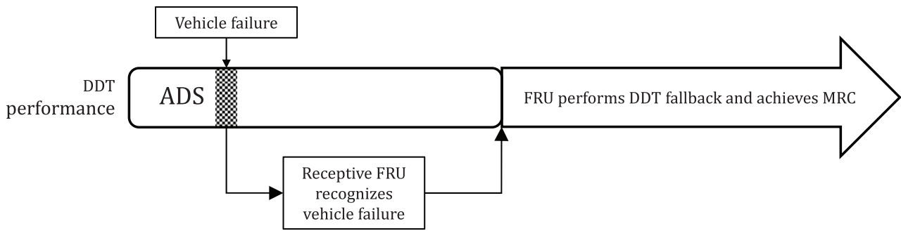
Figure 2 — User performs DDT fallback to MRC
