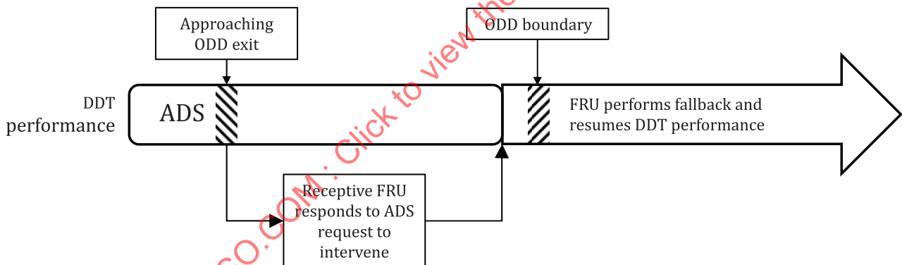
Figure 4 — User resumes DDT as ODD boundary is close
