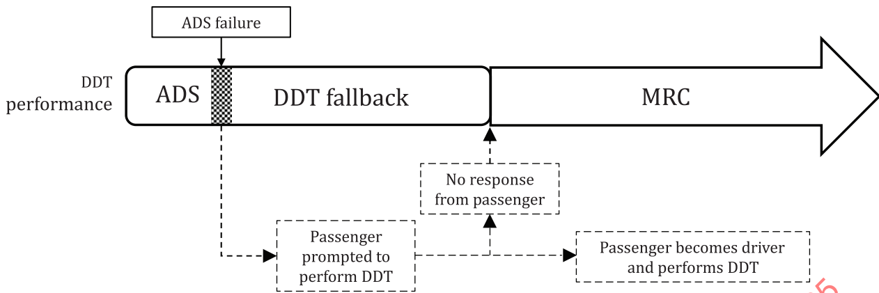
Figure 6 — ADS achieves MRC when user ignored the prompt from ADS on ADS failure
