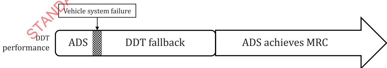
Figure 5 — ADS performs DDT to achieve MRC on vehicle failure
