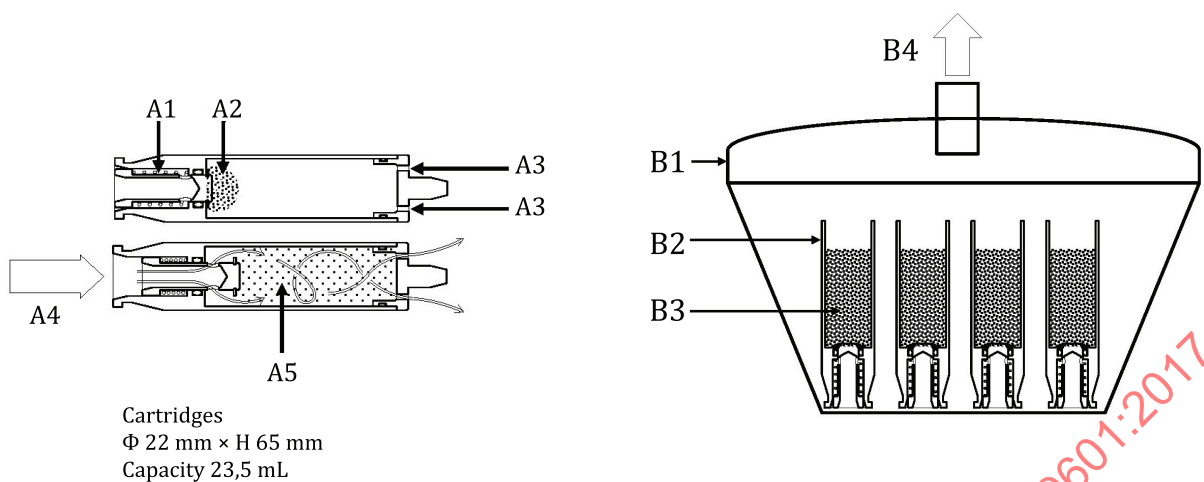
a) Cartridge for direct injection
