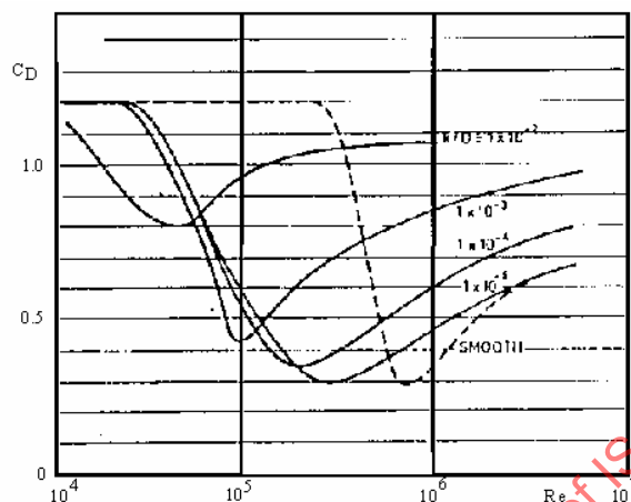
Figure TR.7.3.2.4-10 — Suggested Reynolds dependence in existing guidance [7-37]
