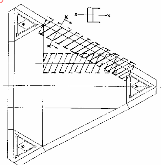
Figure A.8.2-2 — Example division of hull structure into equivalent beams (of different jack-up)
