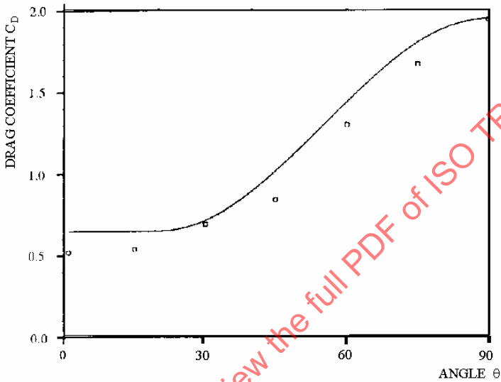
Figure TR.7.C-1 — Comparison of the ISO 19905-1 formulation with model tests, ratio W/D = 1,08 [7-58]
