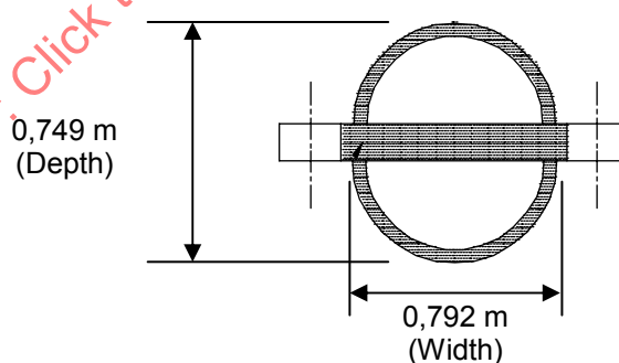
Simplified schematic of leg chord section — Constant cross-section
