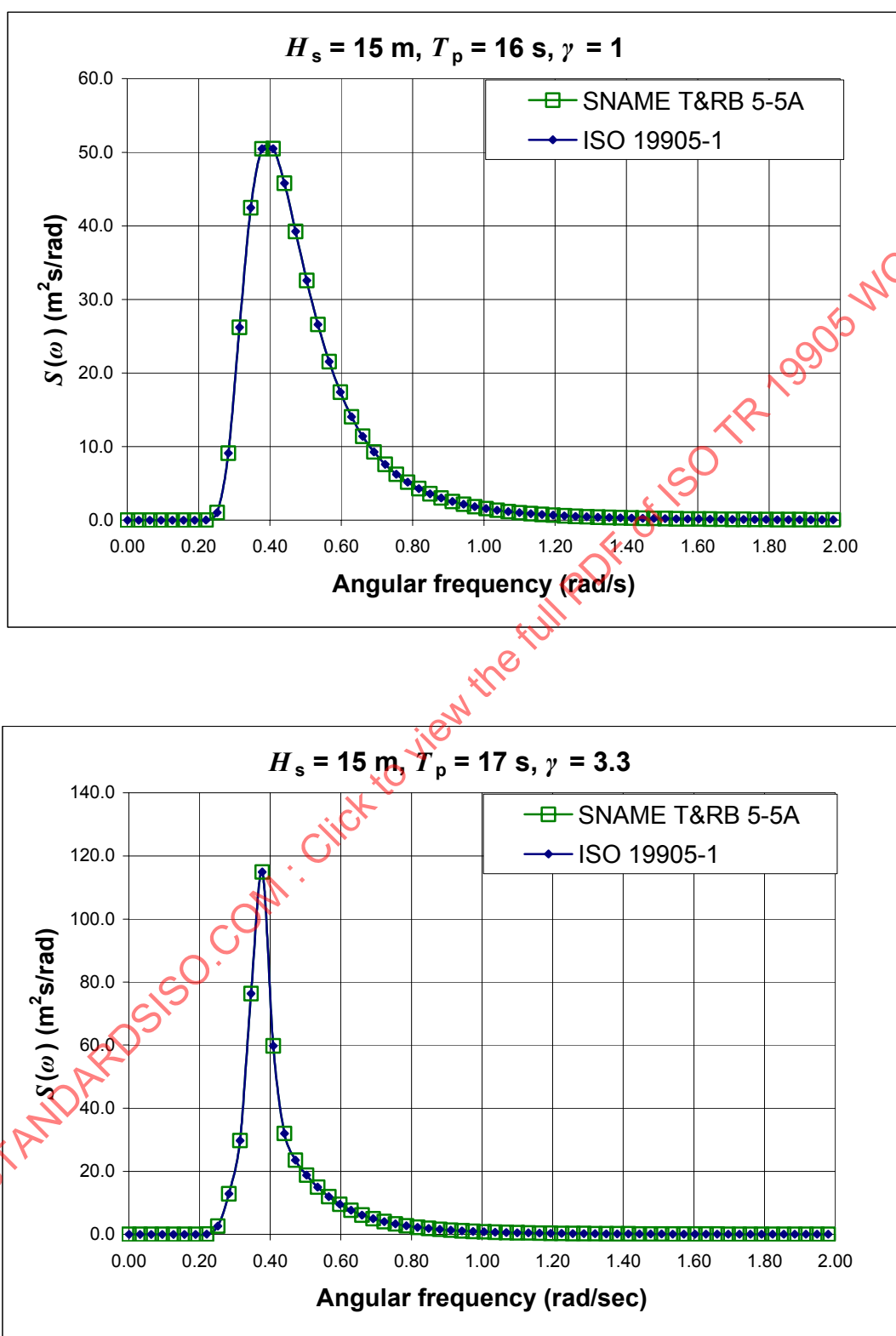
Figure TR.6.4.2.5-1 — Comparison of ISO 19901-1 and SNAME T&R 5-5A wave spectrum formulations
