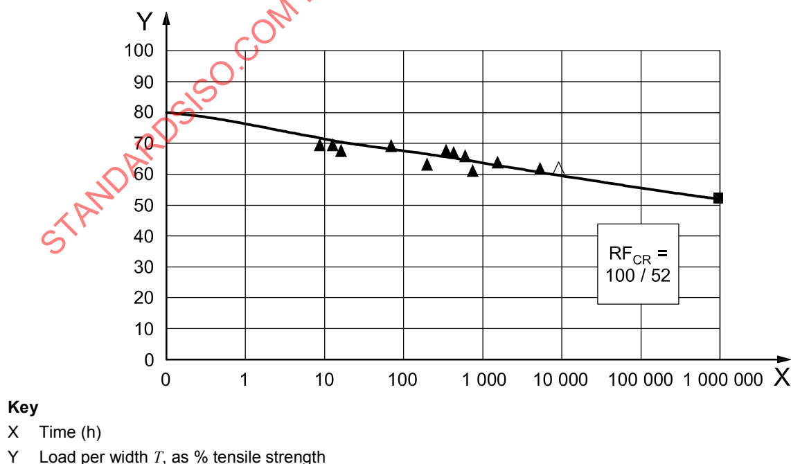
Figure 5 — Creep rupture diagram with straight line fit
