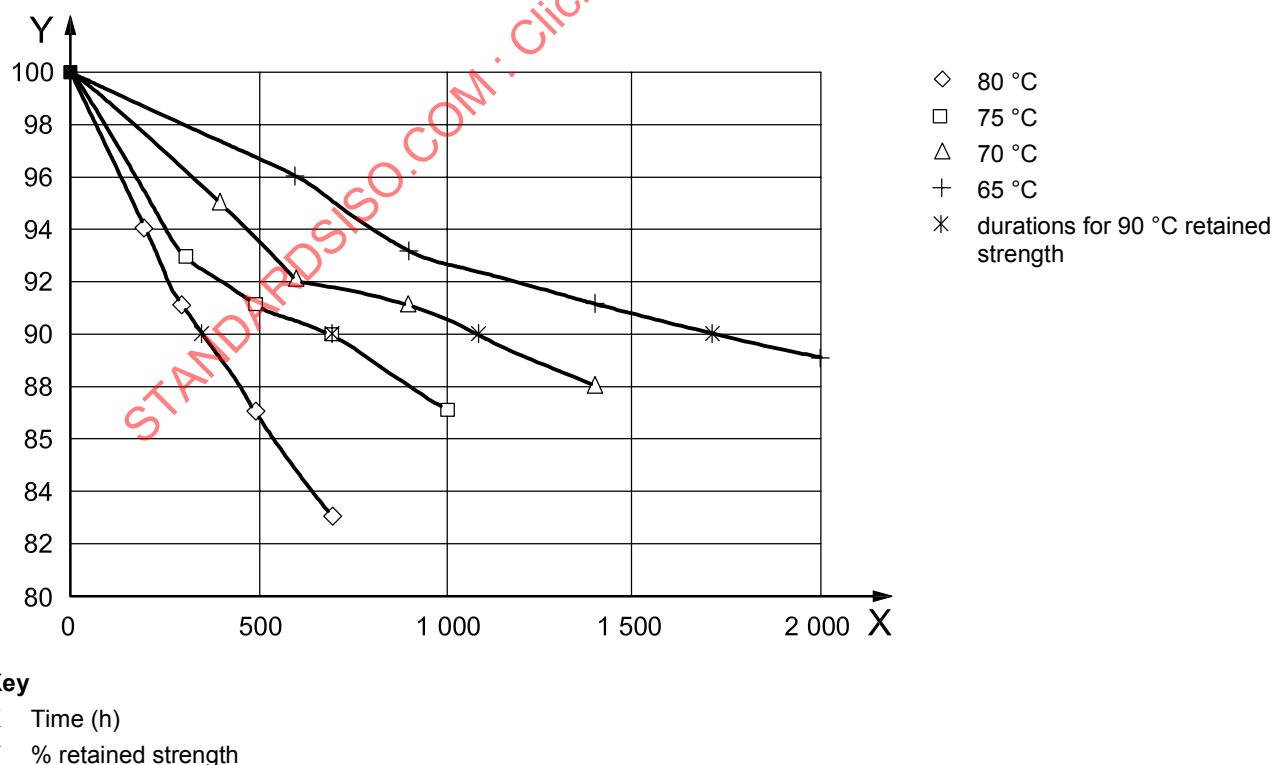
Figure 9 — Reduction in strength at selected temperatures prior to application of Arrhenius' formula
