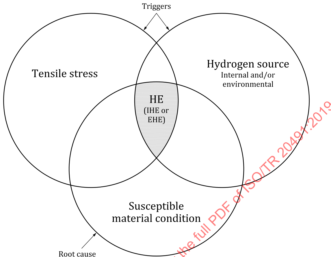
Figure 4 — Confluence of the three necessary conditions for delayed hydrogen embrittlement (HE) failure to occur
